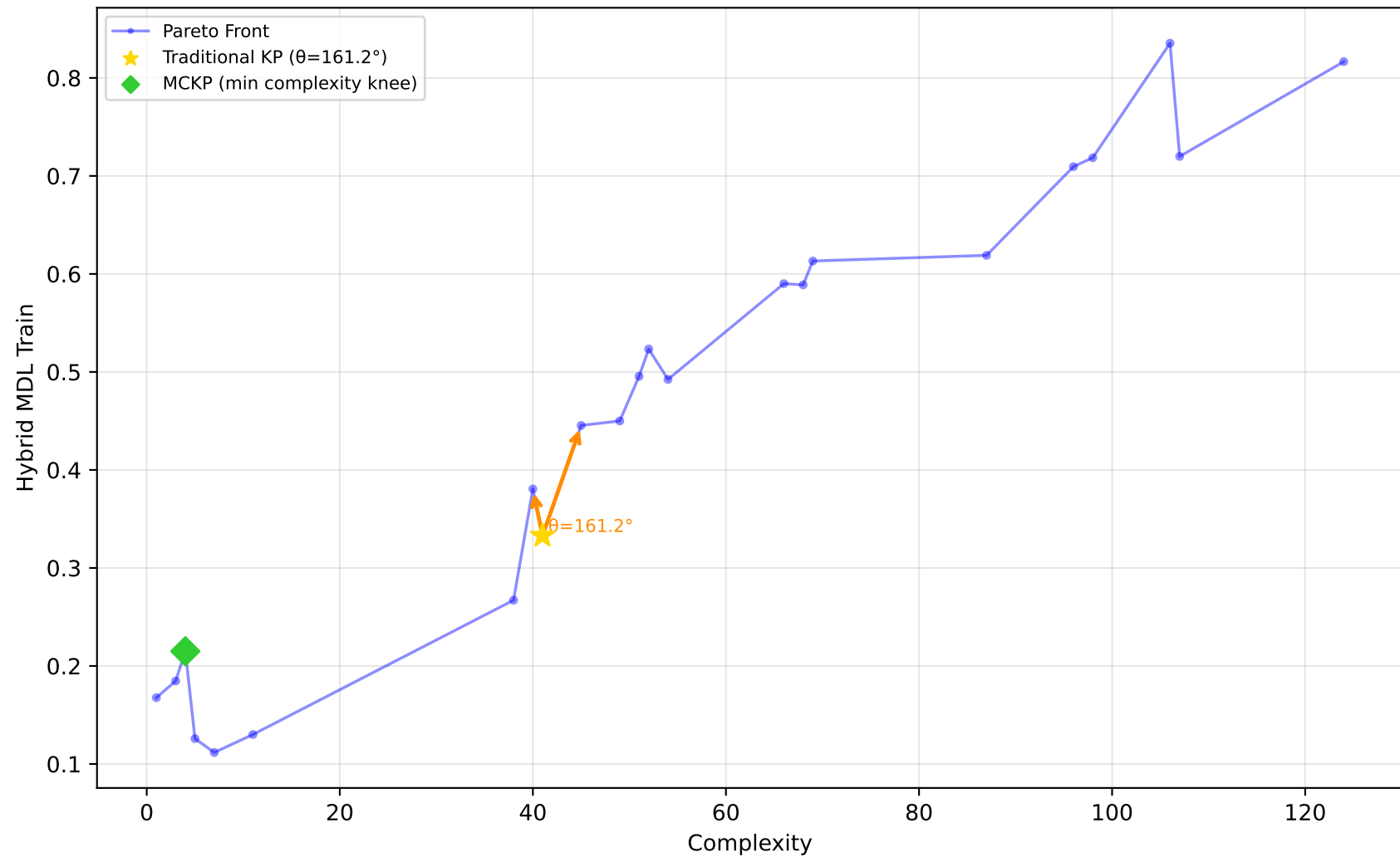
519_vinnie - Run 25 - SVP - Hybrid MDL Train \lambda_1=1.00, \lambda_2=1.00, \lambda_3=1.00 | Difficulty: 1.00 | Method: hmr
