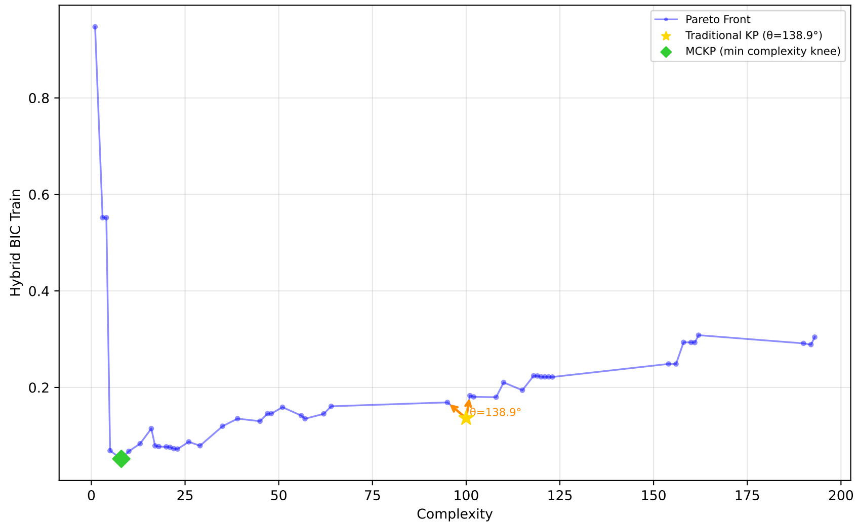
519_vinnie - Run 26 - MVP - Hybrid BIC Train \lambda_1=0.00, \lambda_2=0.10, \lambda_3=0.00 | Difficulty: 0.58 | Method: mckp
