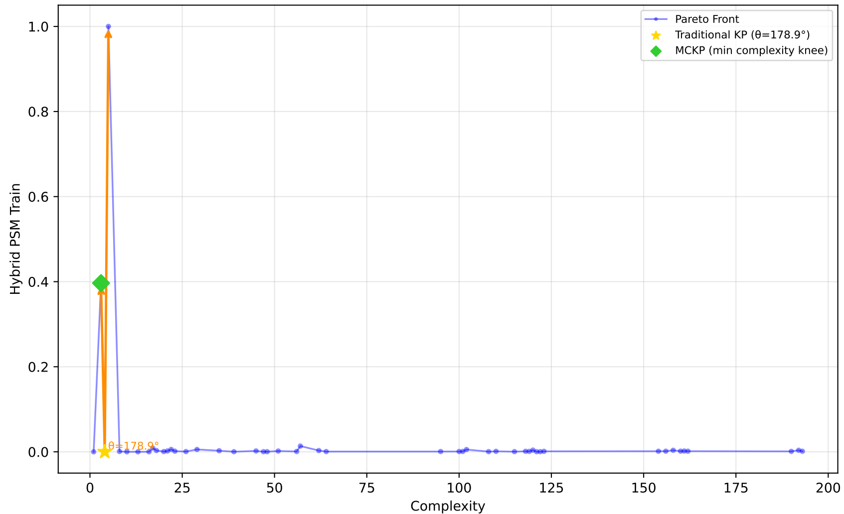
519_vinnie - Run 26 - MVP - Hybrid PSM Train \lambda_1=0.00, \lambda_2=0.10, \lambda_3=0.00 | Difficulty: 0.58 | Method: mckp
