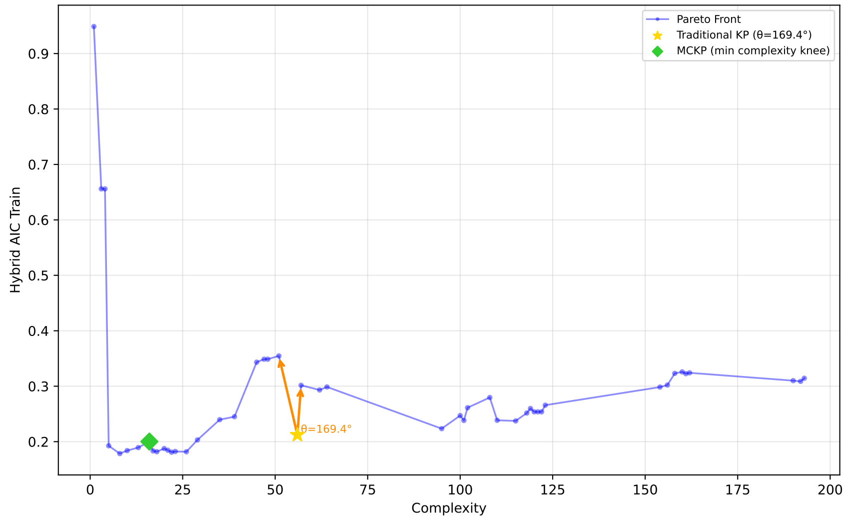
519_vinnie - Run 26 - SVP - Hybrid AIC Train \lambda_1=1.00, \lambda_2=1.00, \lambda_3=1.00 | Difficulty: 0.58 | Method: mckp
