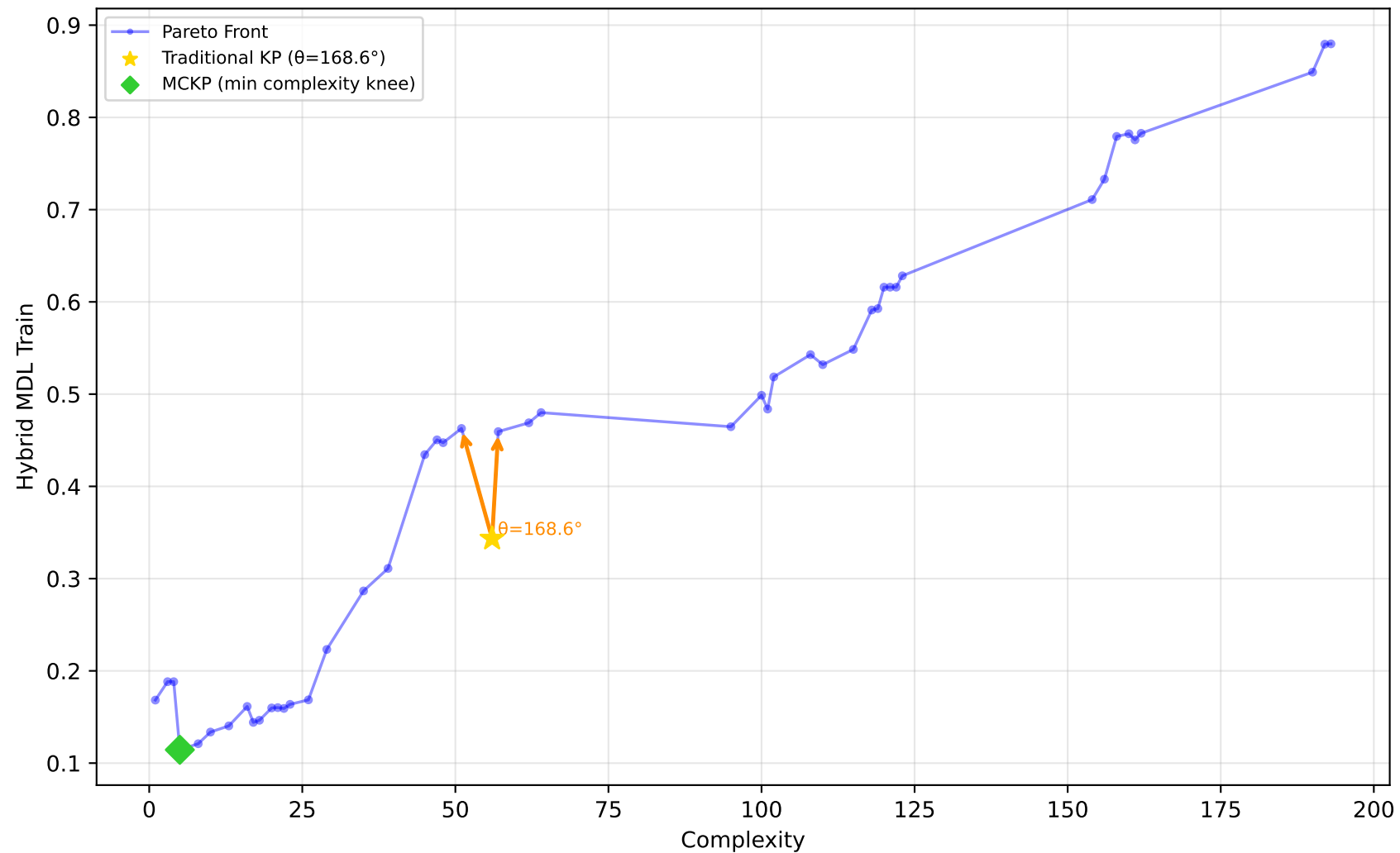
519_vinnie - Run 26 - SVP - Hybrid MDL Train \lambda_1=1.00, \lambda_2=1.00, \lambda_3=1.00 | Difficulty: 0.58 | Method: mckp
