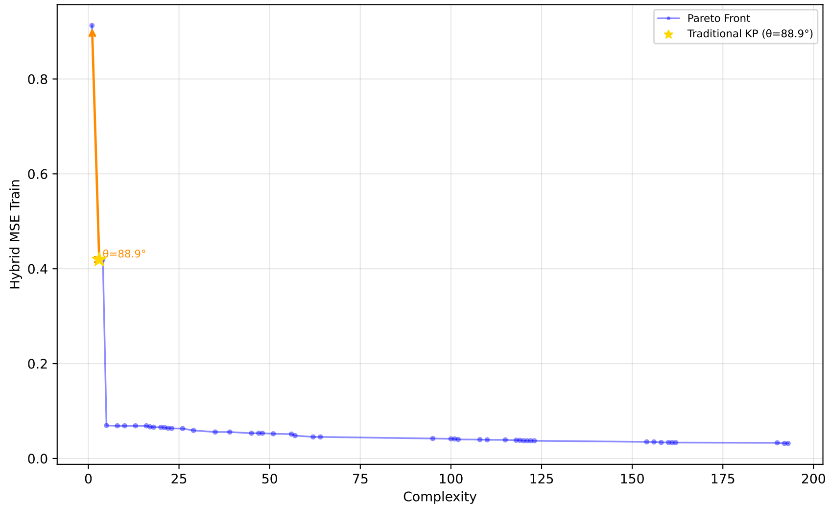
519_vinnie - Run 26 - SVP - Hybrid MSE Train \lambda_1=0.00, \lambda_2=0.00, \lambda_3=0.00 | Difficulty: 0.58 | Method: mckp
