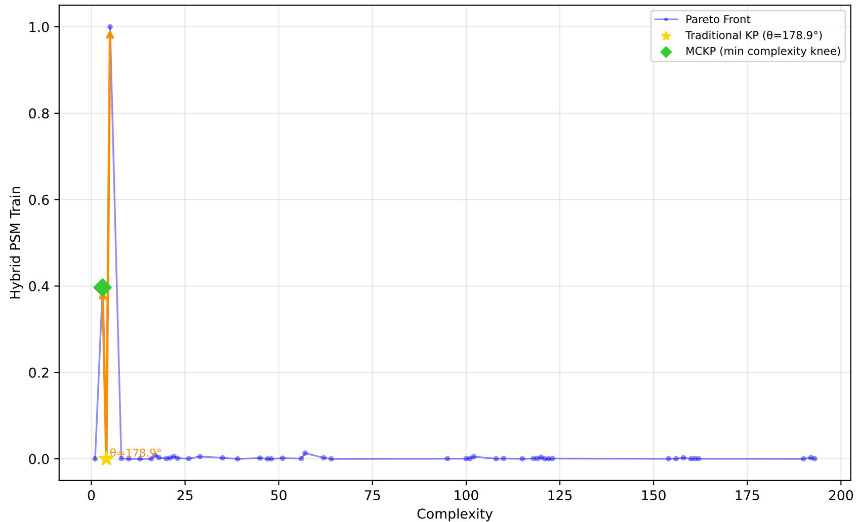
519_vinnie - Run 26 - SVP - Hybrid PSM Train \lambda_1=0.00, \lambda_2=0.00, \lambda_3=0.00 | Difficulty: 0.58 | Method: mckp
