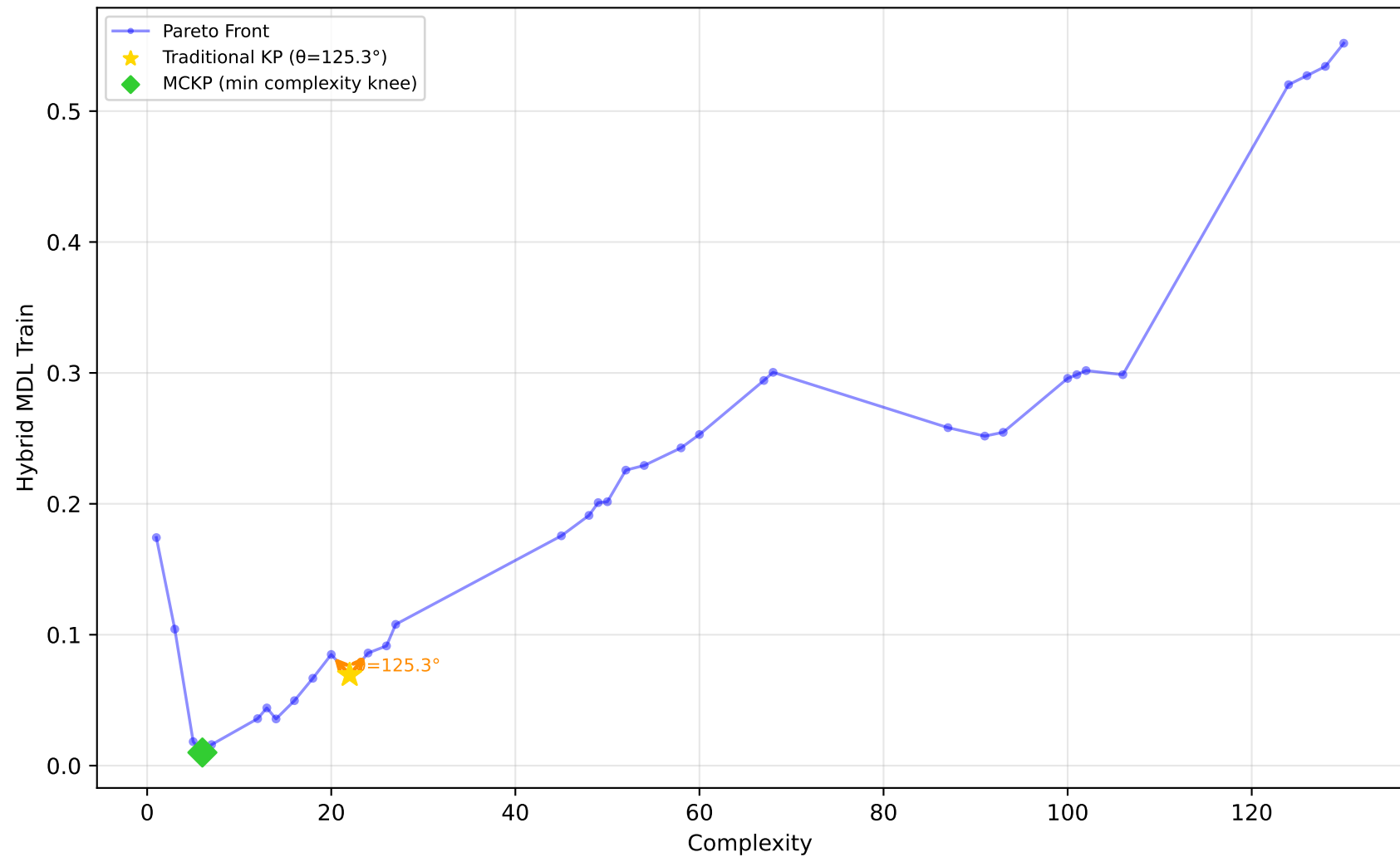
519_vinnie - Run 27 - MVP - Hybrid MDL Train \lambda_1=0.00, \lambda_2=0.10, \lambda_3=0.00 | Difficulty: 0.58 | Method: mckp
