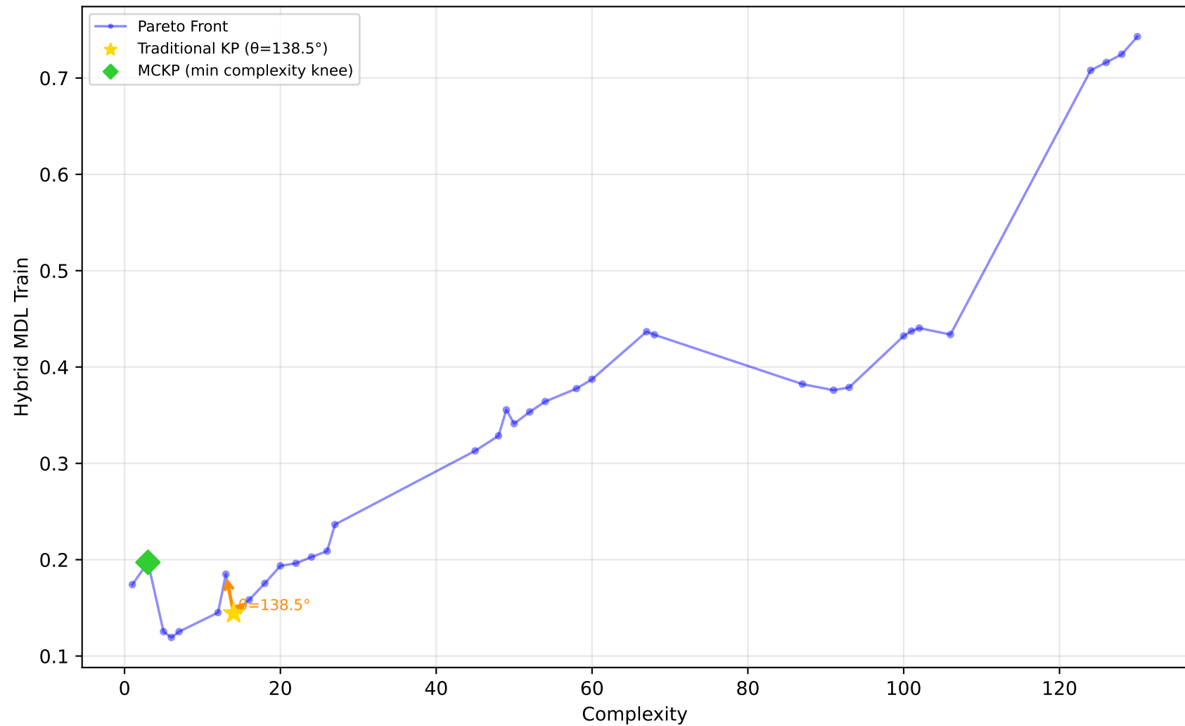
519_vinnie - Run 27 - MVP - Hybrid MDL Train \lambda_1=1.00, \lambda_2=0.00, \lambda_3=1.00 | Difficulty: 0.58 | Method: mckp
