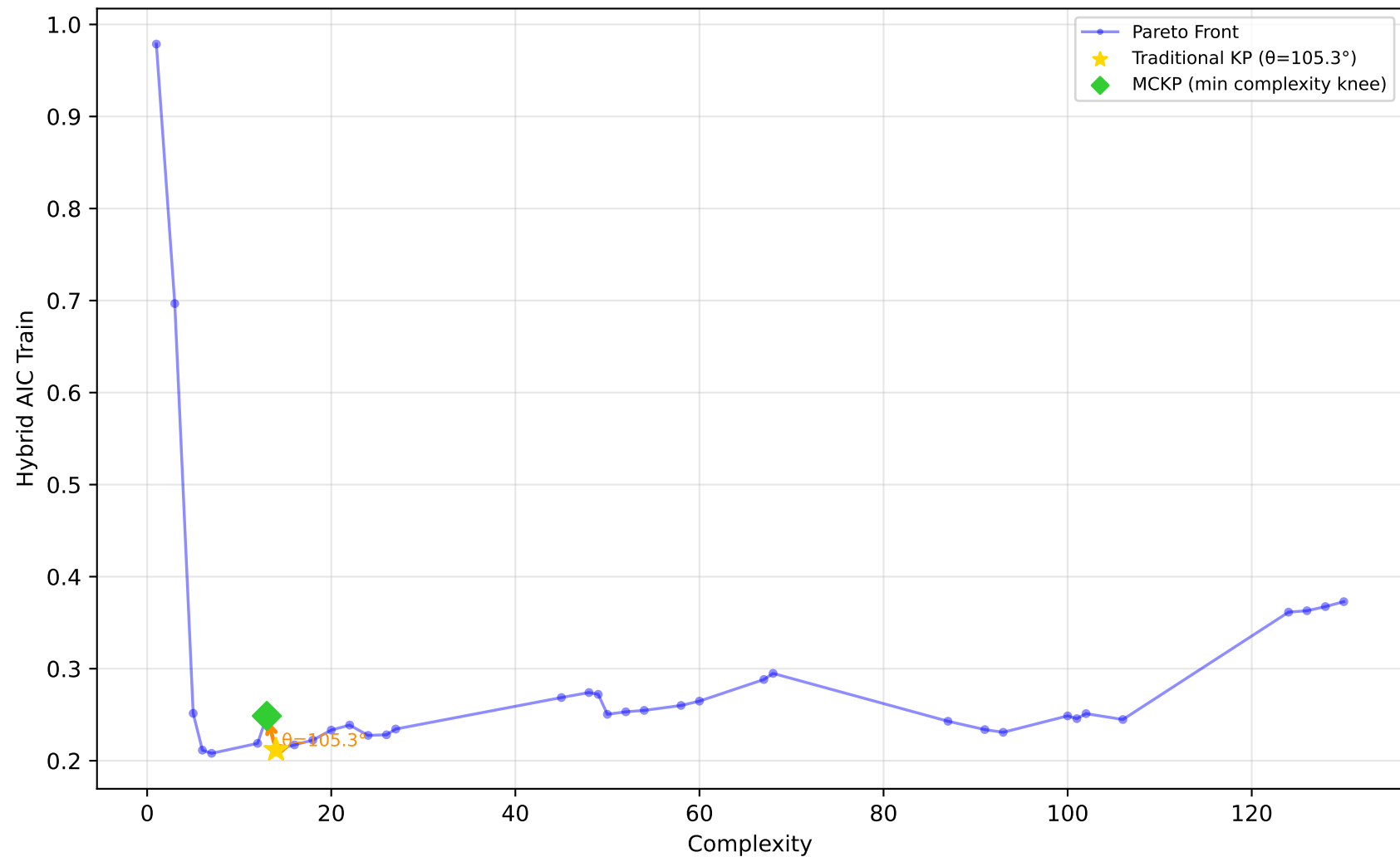
519_vinnie - Run 27 - SVP - Hybrid AIC Train \lambda_1=1.00, \lambda_2=1.00, \lambda_3=1.00 | Difficulty: 0.58 | Method: mckp
