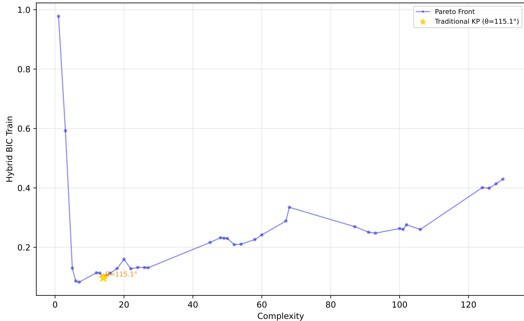
519_vinnie - Run 27 - SVP - Hybrid BIC Train \lambda_1=0.00, \lambda_2=0.00, \lambda_3=0.00 | Difficulty: 0.58 | Method: mckp
