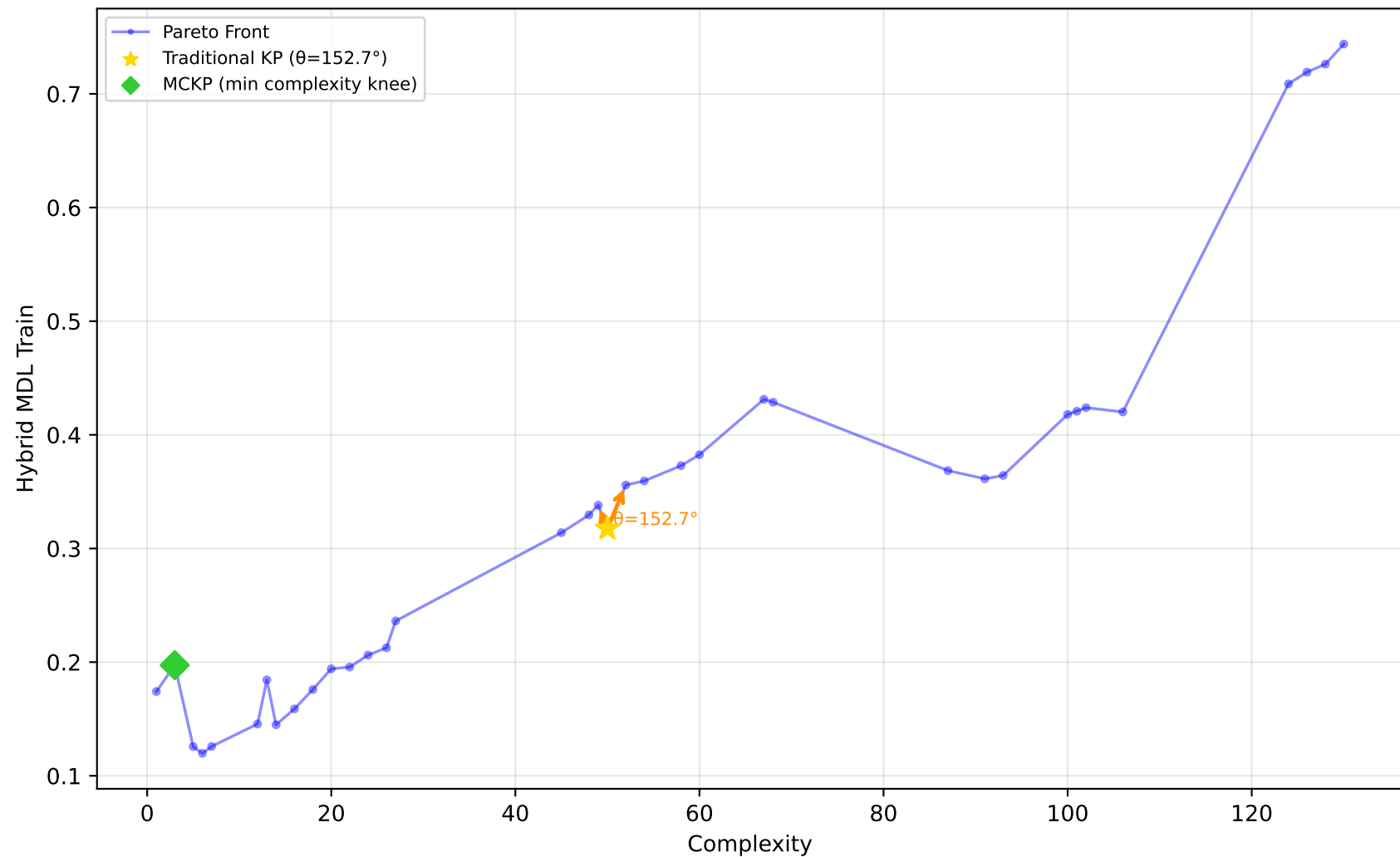
519_vinnie - Run 27 - SVP - Hybrid MDL Train \lambda_1=1.00, \lambda_2=1.00, \lambda_3=1.00 | Difficulty: 0.58 | Method: mckp
