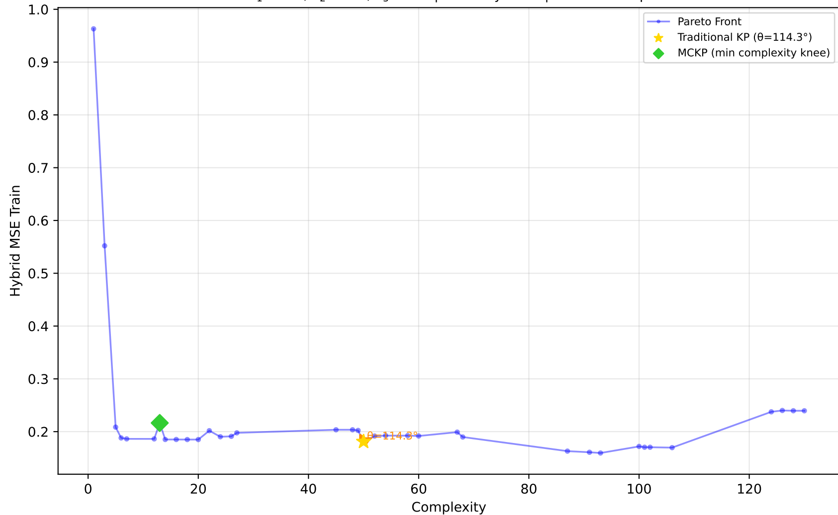
519_vinnie - Run 27 - SVP - Hybrid MSE Train \lambda_1=1.00, \lambda_2=1.00, \lambda_3=1.00 | Difficulty: 0.58 | Method: mckp
