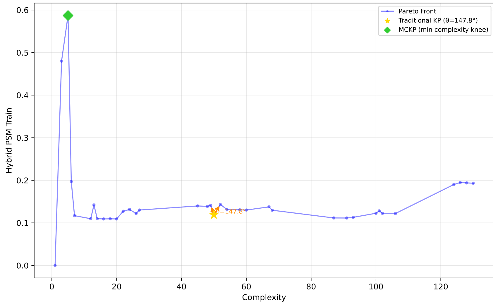
519_vinnie - Run 27 - SVP - Hybrid PSM Train \lambda_1=1.00, \lambda_2=1.00, \lambda_3=1.00 | Difficulty: 0.58 | Method: mckp
