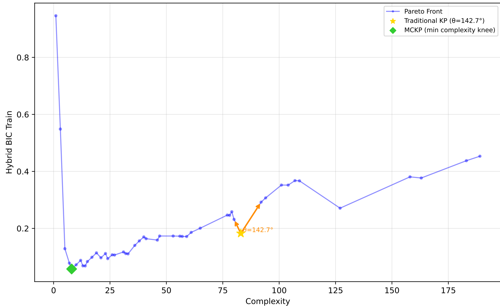
519_vinnie - Run 28 - SVP - Hybrid BIC Train \lambda_1=0.00, \lambda_2=0.00, \lambda_3=0.00 | Difficulty: 0.47 | Method: mckp
