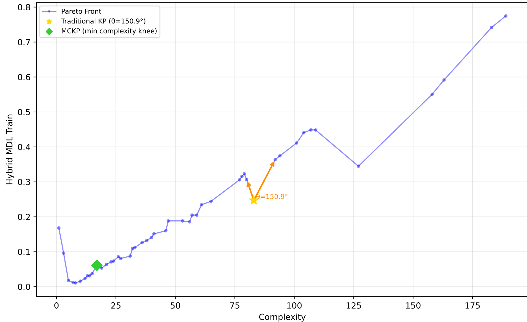
519_vinnie - Run 28 - SVP - Hybrid MDL Train \lambda_1=0.00, \lambda_2=0.00, \lambda_3=0.00 | Difficulty: 0.47 | Method: mckp
