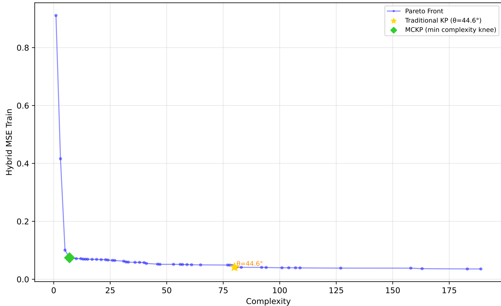
519_vinnie - Run 28 - SVP - Hybrid MSE Train \lambda_1=0.00, \lambda_2=0.00, \lambda_3=0.00 | Difficulty: 0.47 | Method: mckp
