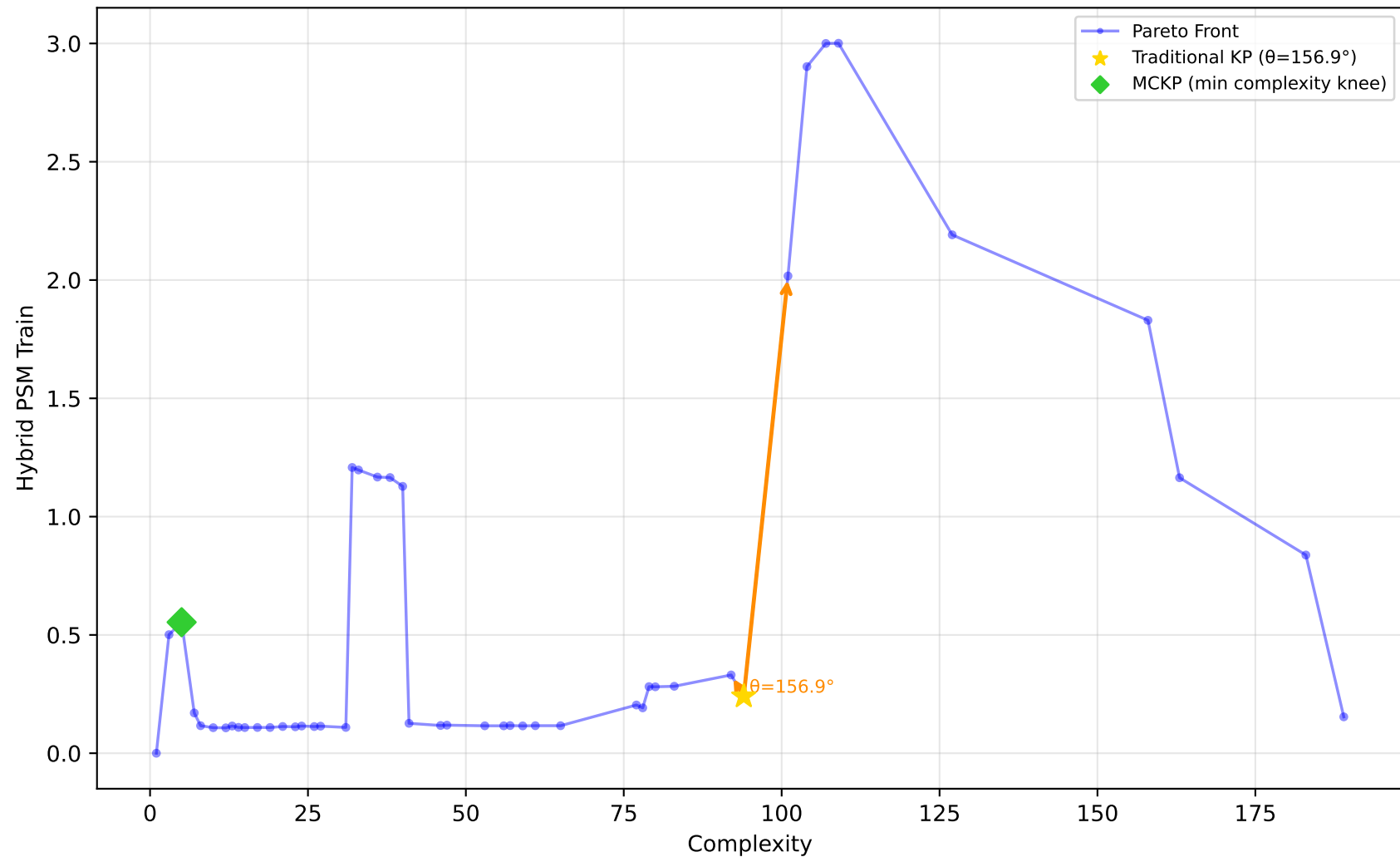
519_vinnie - Run 28 - SVP - Hybrid PSM Train \lambda_1=1.00, \lambda_2=1.00, \lambda_3=1.00 | Difficulty: 0.47 | Method: mckp
