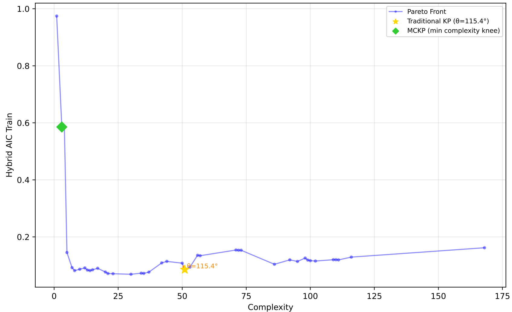
519_vinnie - Run 29 - MVP - Hybrid AIC Train \lambda_1=0.00, \lambda_2=0.10, \lambda_3=0.00 | Difficulty: 1.00 | Method: hmr
