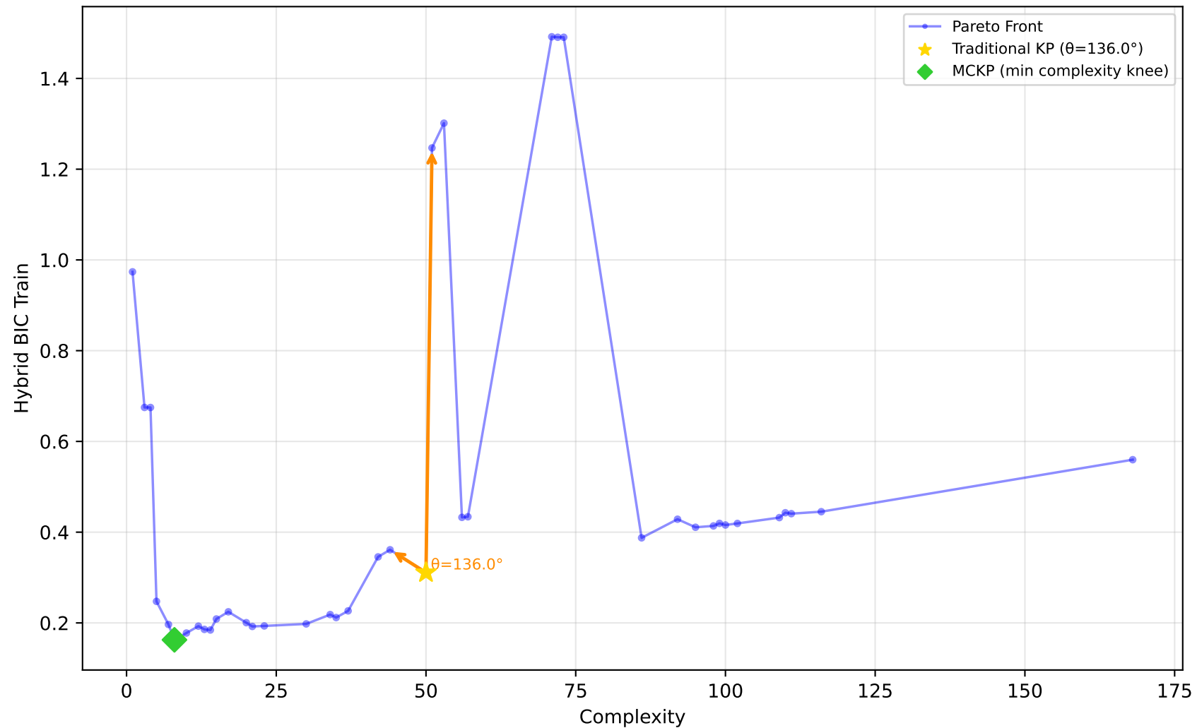
519_vinnie - Run 29 - MVP - Hybrid BIC Train \lambda_1=1.00, \lambda_2=0.00, \lambda_3=1.00 | Difficulty: 1.00 | Method: hmr
