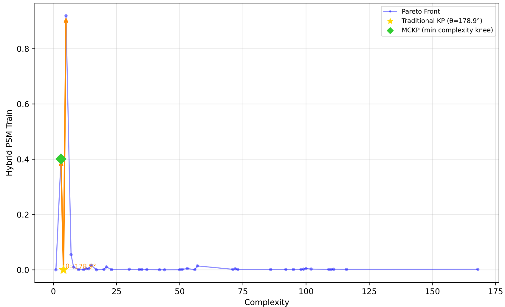
519_vinnie - Run 29 - MVP - Hybrid PSM Train \lambda_1=0.00, \lambda_2=0.10, \lambda_3=0.00 | Difficulty: 1.00 | Method: hmr
