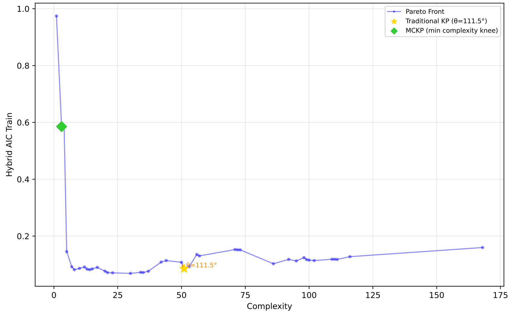
519_vinnie - Run 29 - SVP - Hybrid AIC Train \lambda_1=0.00, \lambda_2=0.00, \lambda_3=0.00 | Difficulty: 1.00 | Method: hmr
