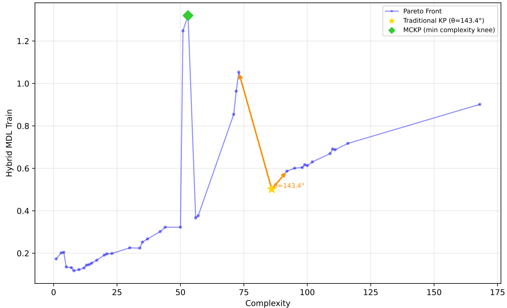
519_vinnie - Run 29 - SVP - Hybrid MDL Train \lambda_1=1.00, \lambda_2=1.00, \lambda_3=1.00 | Difficulty: 1.00 | Method: hmr
