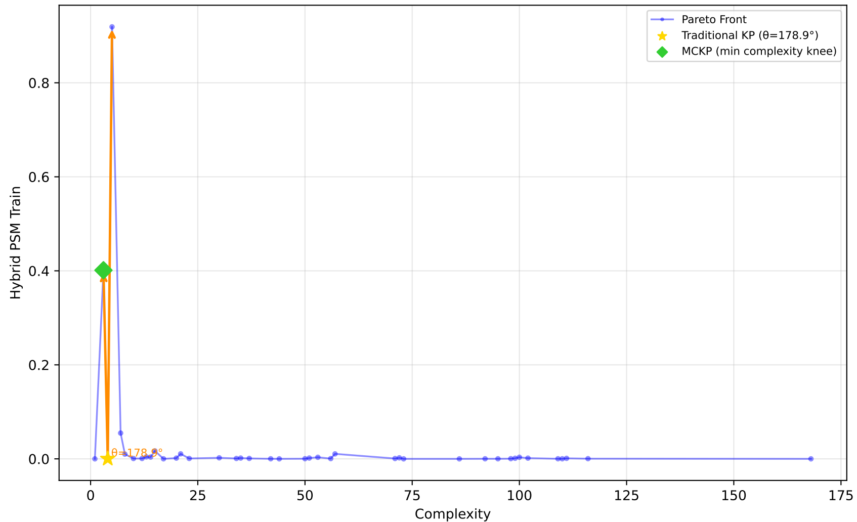
519_vinnie - Run 29 - SVP - Hybrid PSM Train \lambda_1=0.00, \lambda_2=0.00, \lambda_3=0.00 | Difficulty: 1.00 | Method: hmr
