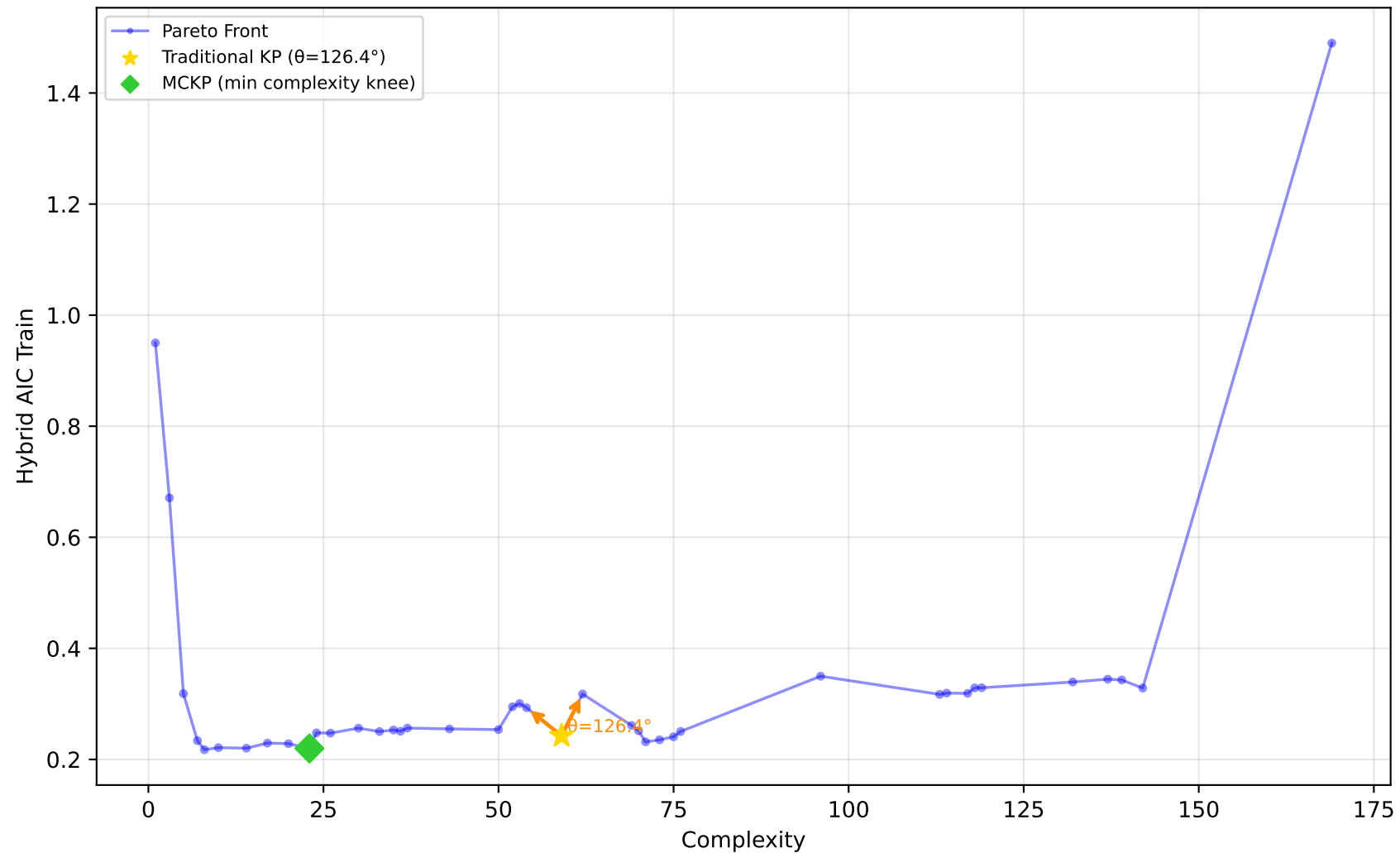
519_vinnie - Run 2 - MVP - Hybrid AIC Train \lambda_1=1.00, \lambda_2=0.00, \lambda_3=1.00 | Difficulty: 0.77 | Method: hmr
