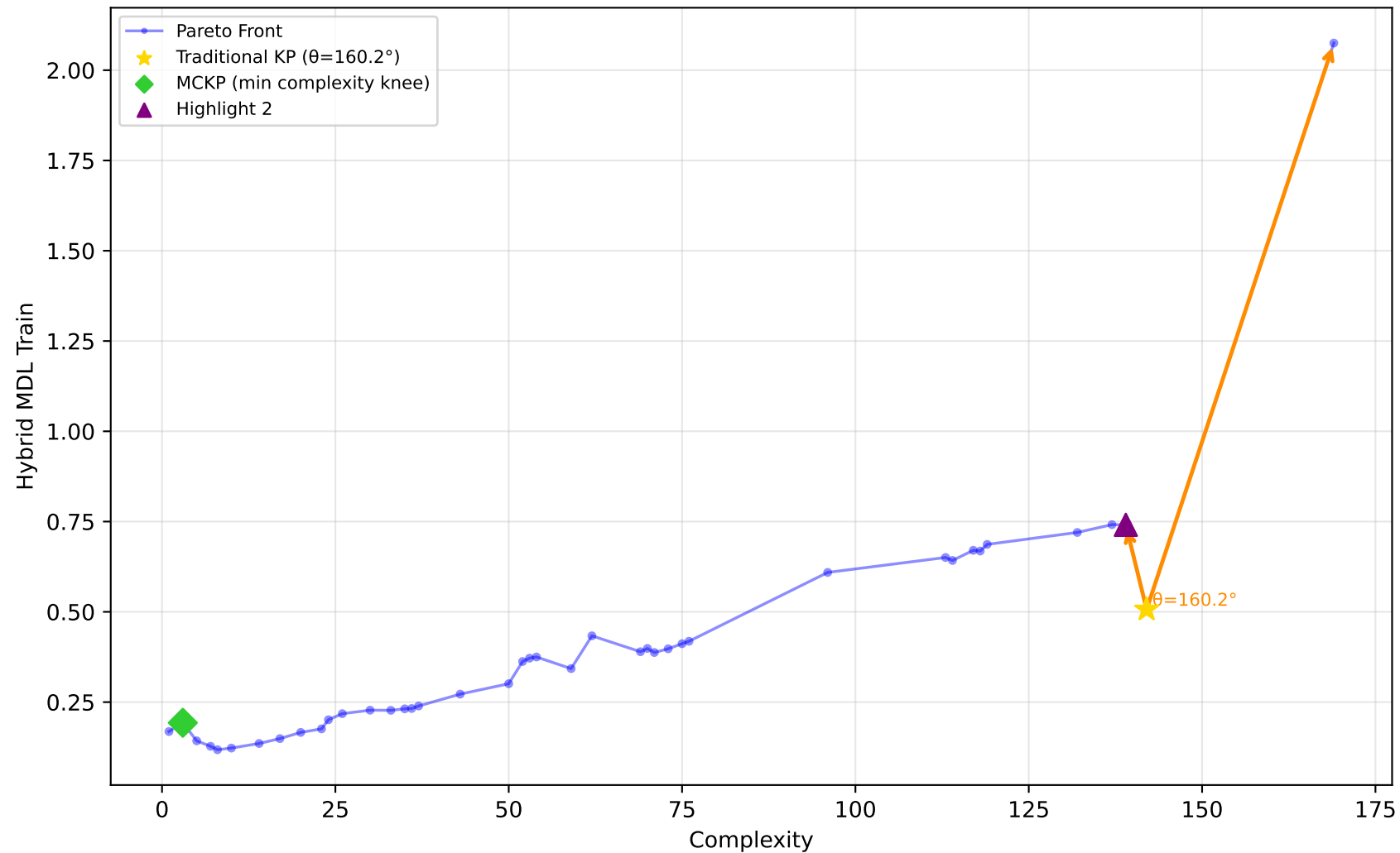
519_vinnie - Run 2 - MVP - Hybrid MDL Train \lambda_1=1.00, \lambda_2=0.00, \lambda_3=1.00 | Difficulty: 0.77 | Method: hmr
