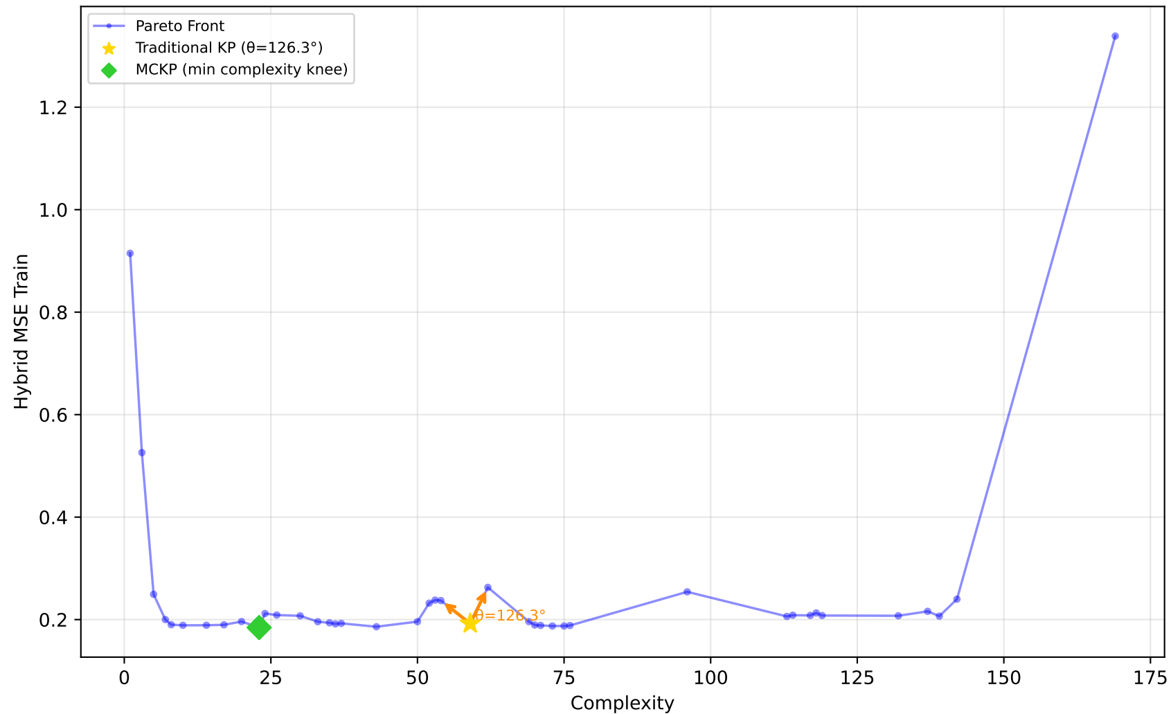
519_vinnie - Run 2 - MVP - Hybrid MSE Train \lambda_1=1.00, \lambda_2=0.00, \lambda_3=1.00 | Difficulty: 0.77 | Method: hmr
