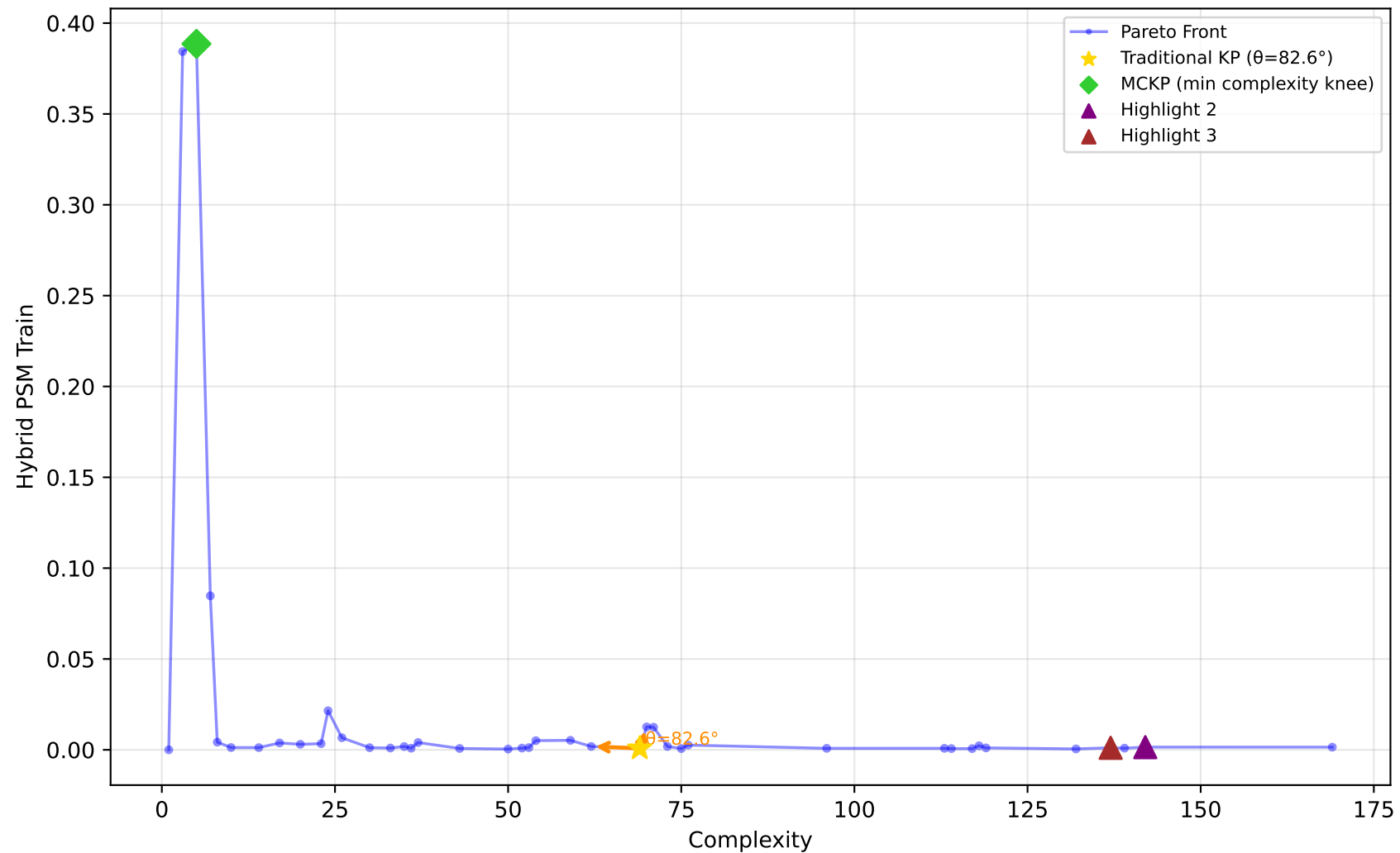
519_vinnie - Run 2 - MVP - Hybrid PSM Train \lambda_1=0.00, \lambda_2=0.10, \lambda_3=0.00 | Difficulty: 0.77 | Method: hmr
