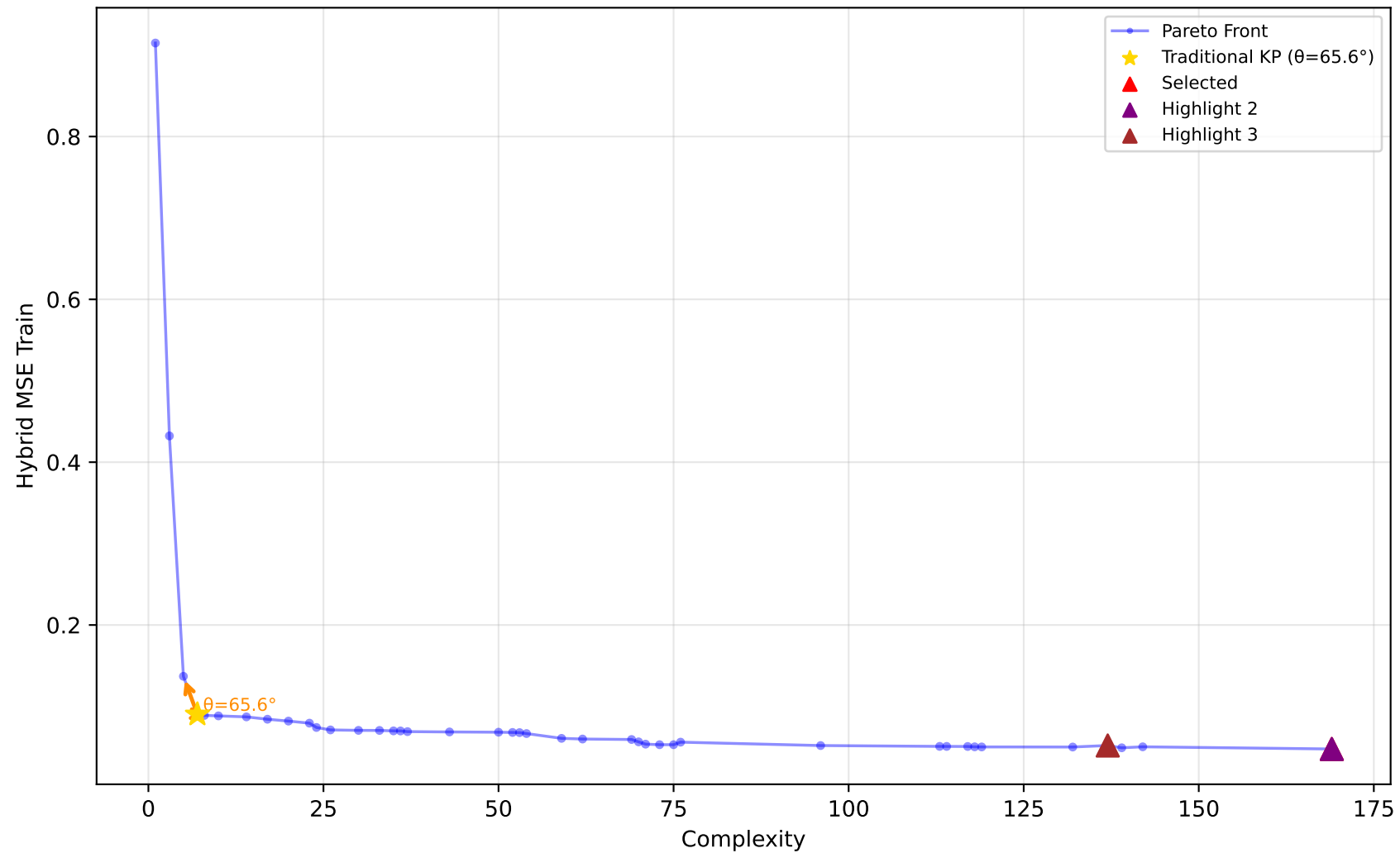
519_vinnie - Run 2 - SVP - Hybrid MSE Train \lambda_1=0.00, \lambda_2=0.00, \lambda_3=0.00 | Difficulty: 0.77 | Method: hmr
