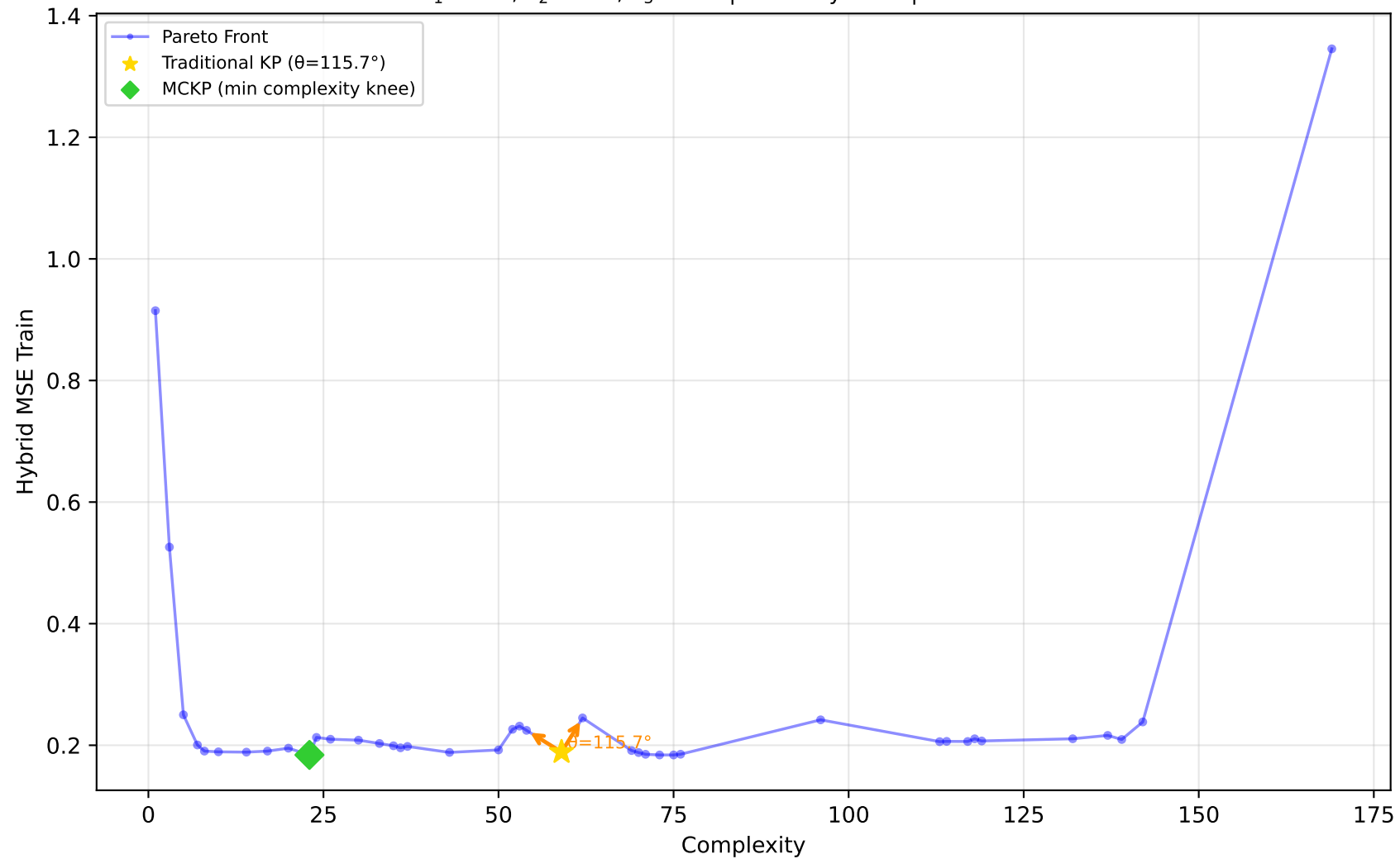
519_vinnie - Run 2 - SVP - Hybrid MSE Train \lambda_1=1.00, \lambda_2=1.00, \lambda_3=1.00 | Difficulty: 0.77 | Method: hmr
