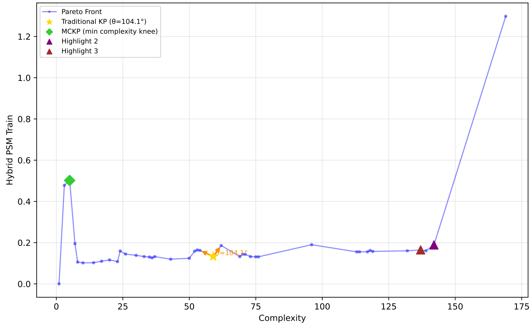
519_vinnie - Run 2 - SVP - Hybrid PSM Train \lambda_1=1.00, \lambda_2=1.00, \lambda_3=1.00 | Difficulty: 0.77 | Method: hmr
