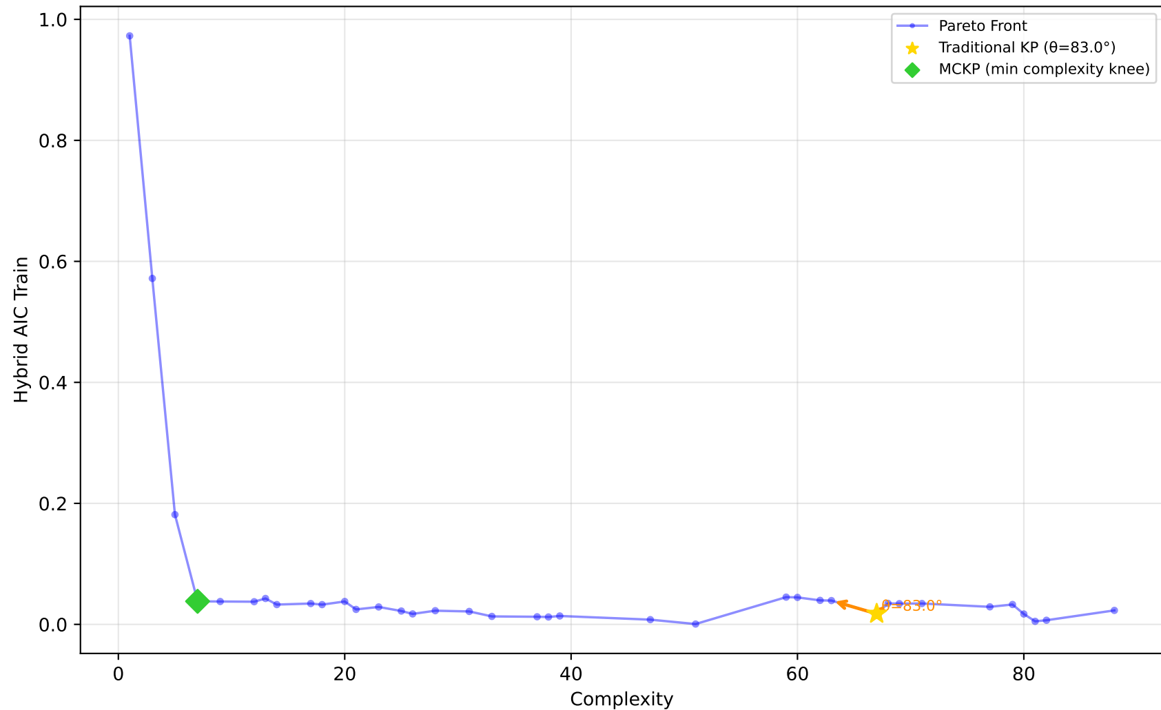
519_vinnie - Run 30 - MVP - Hybrid AIC Train \lambda_1=0.00, \lambda_2=0.10, \lambda_3=0.00 | Difficulty: 0.52 | Method: mckp
