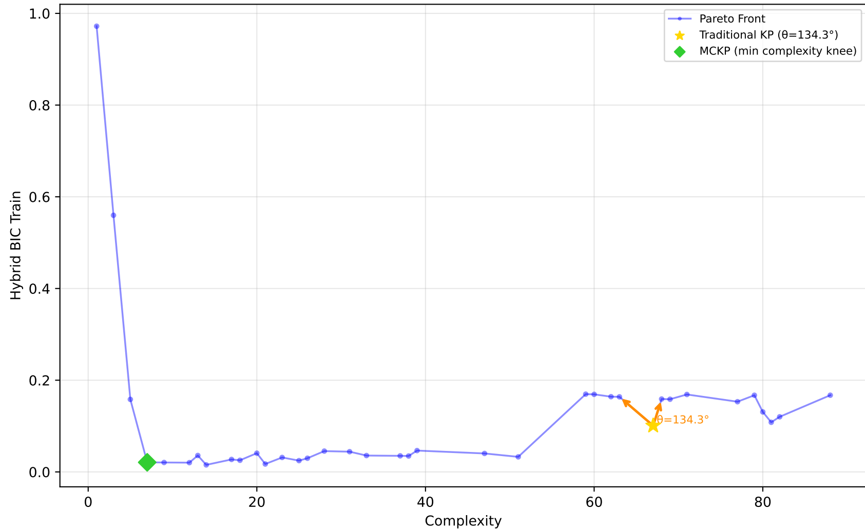
519_vinnie - Run 30 - MVP - Hybrid BIC Train \lambda_1=0.00, \lambda_2=0.10, \lambda_3=0.00 | Difficulty: 0.52 | Method: mckp
