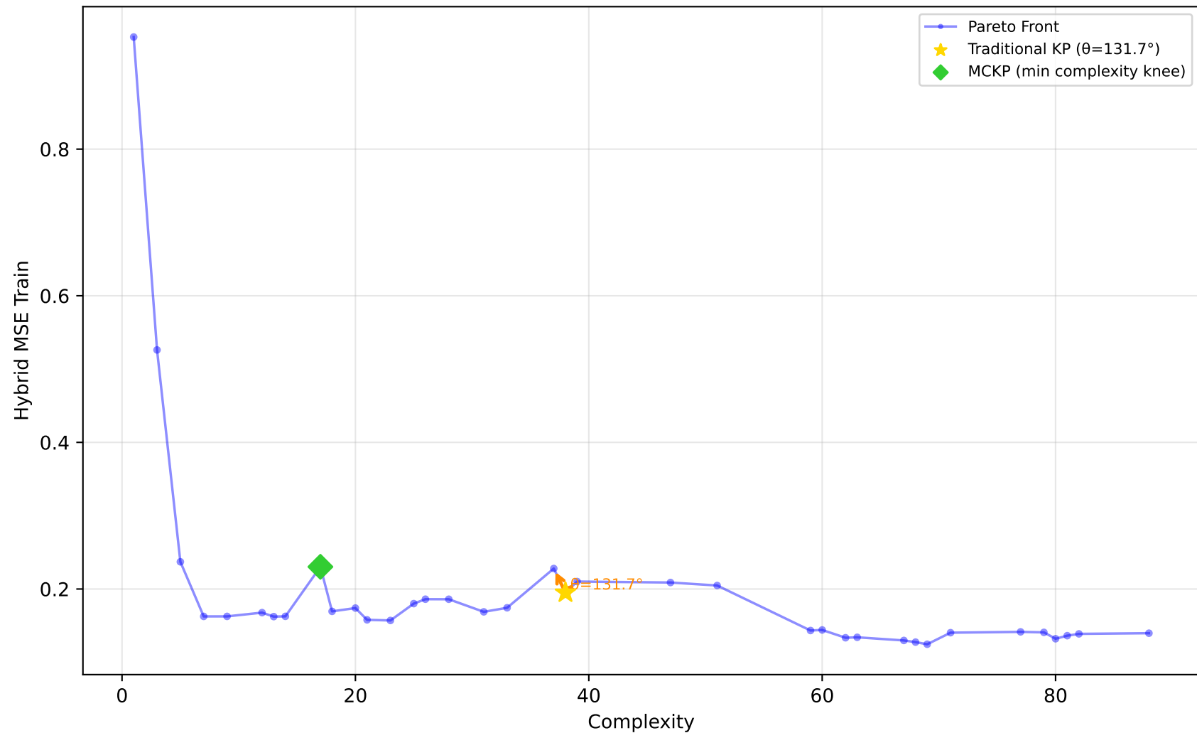
519_vinnie - Run 30 - MVP - Hybrid MSE Train \lambda_1=1.00, \lambda_2=0.00, \lambda_3=1.00 | Difficulty: 0.52 | Method: mckp
