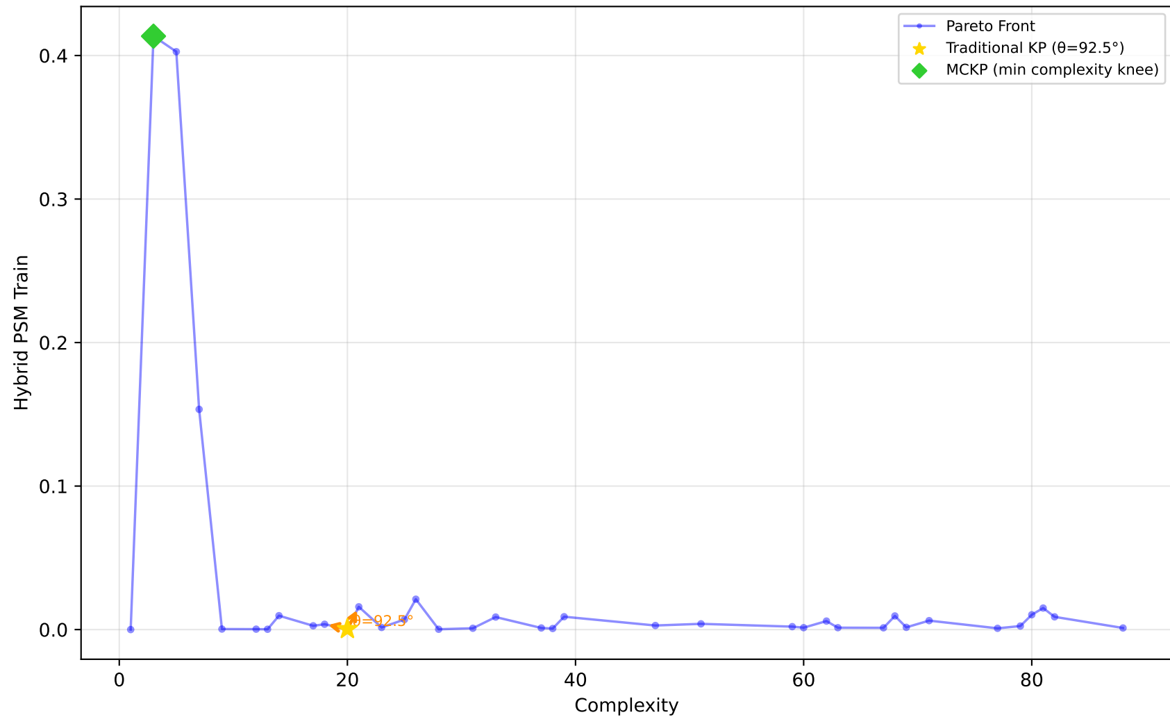
519_vinnie - Run 30 - MVP - Hybrid PSM Train \lambda_1=0.00, \lambda_2=0.10, \lambda_3=0.00 | Difficulty: 0.52 | Method: mckp
