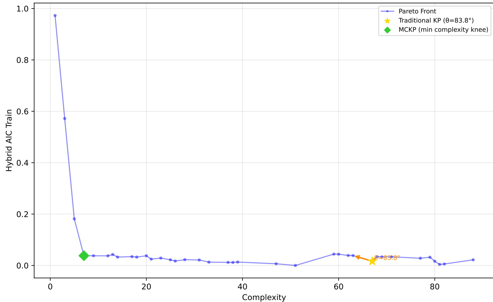
519_vinnie - Run 30 - SVP - Hybrid AIC Train \lambda_1=0.00, \lambda_2=0.00, \lambda_3=0.00 | Difficulty: 0.52 | Method: mckp
