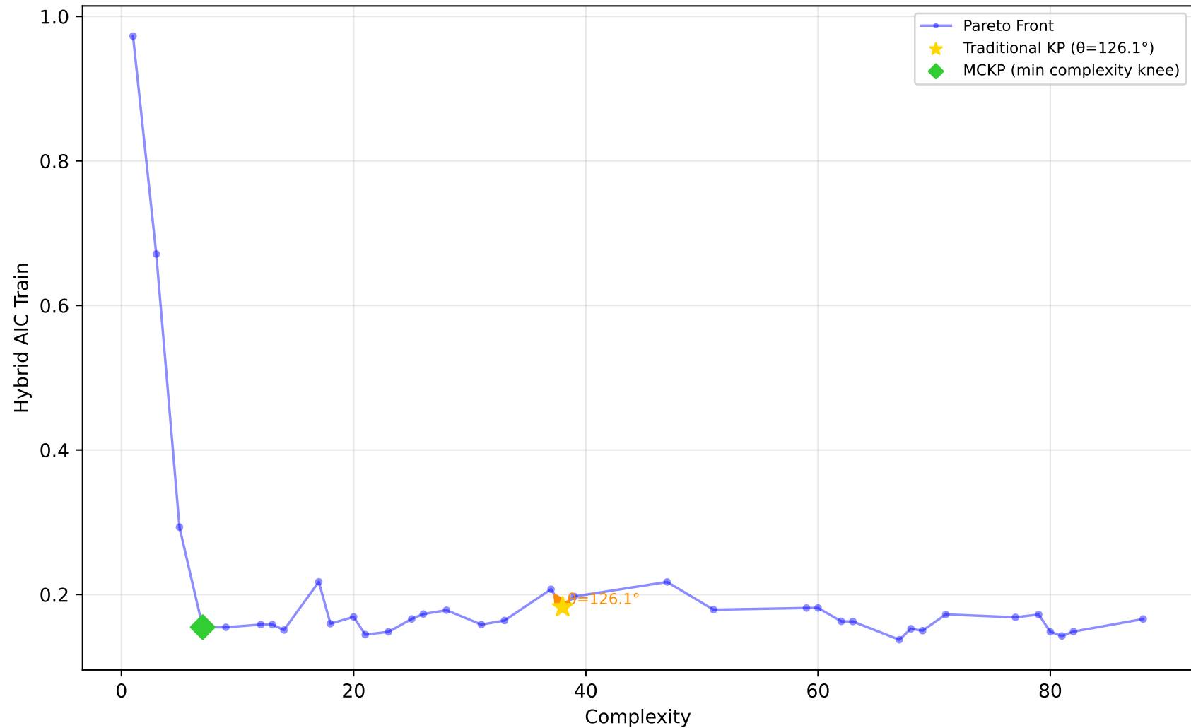
519_vinnie - Run 30 - SVP - Hybrid AIC Train \lambda_1=1.00, \lambda_2=1.00, \lambda_3=1.00 | Difficulty: 0.52 | Method: mckp
