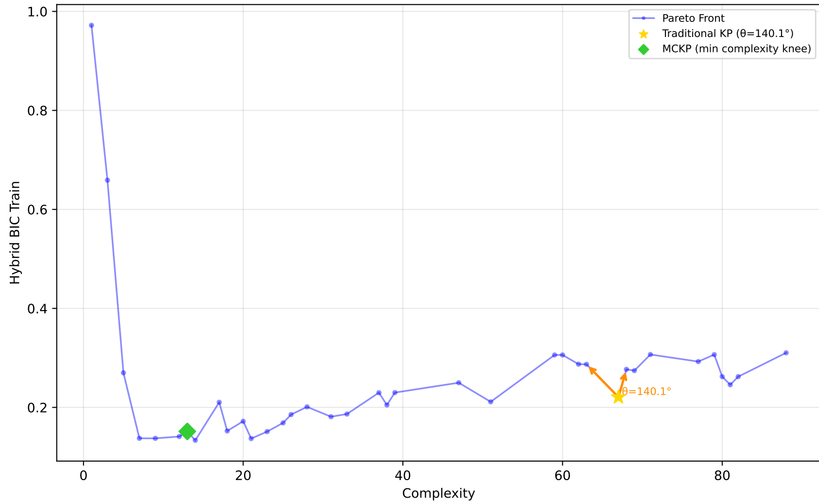
519_vinnie - Run 30 - SVP - Hybrid BIC Train \lambda_1=1.00, \lambda_2=1.00, \lambda_3=1.00 | Difficulty: 0.52 | Method: mckp
