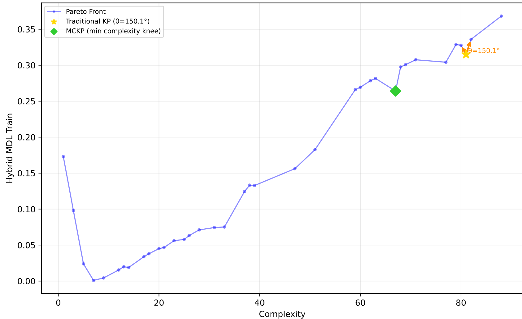
519_vinnie - Run 30 - SVP - Hybrid MDL Train \lambda_1=0.00, \lambda_2=0.00, \lambda_3=0.00 | Difficulty: 0.52 | Method: mckp
