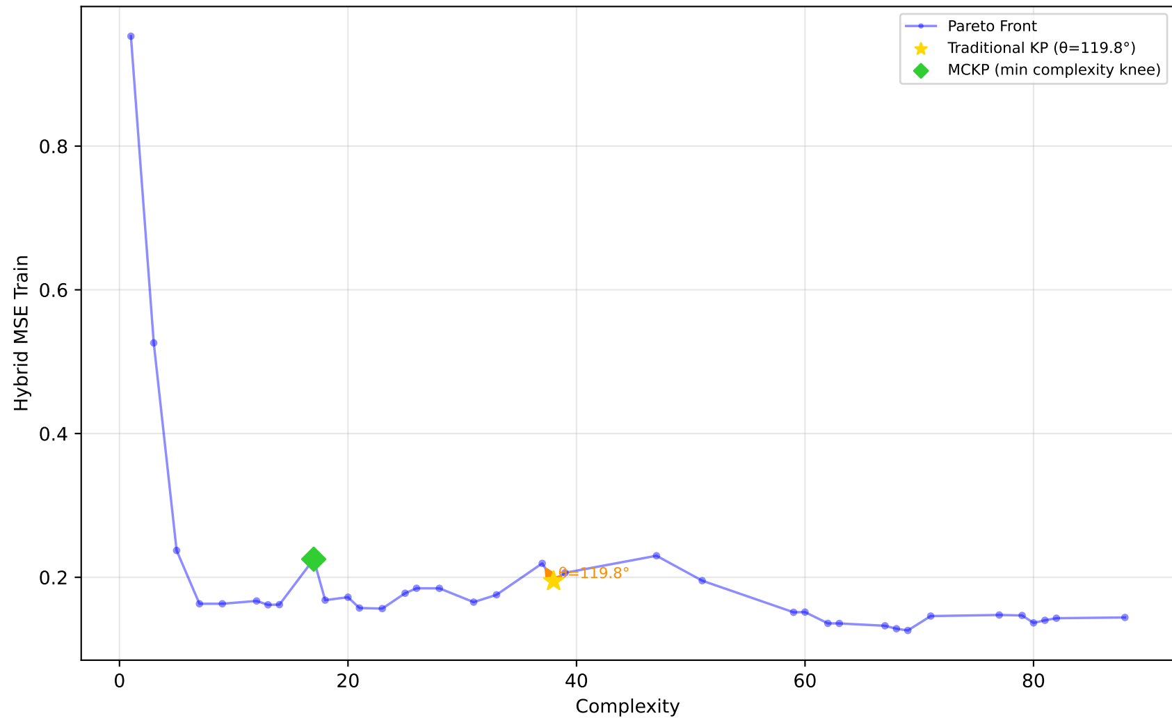
519_vinnie - Run 30 - SVP - Hybrid MSE Train \lambda_1=1.00, \lambda_2=1.00, \lambda_3=1.00 | Difficulty: 0.52 | Method: mckp
