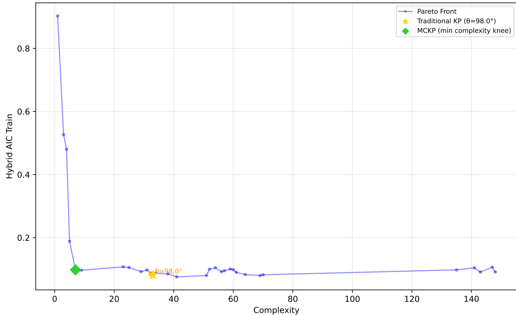
519_vinnie - Run 3 - MVP - Hybrid AIC Train \lambda_1=0.00, \lambda_2=0.10, \lambda_3=0.00 | Difficulty: 1.00 | Method: hmr
