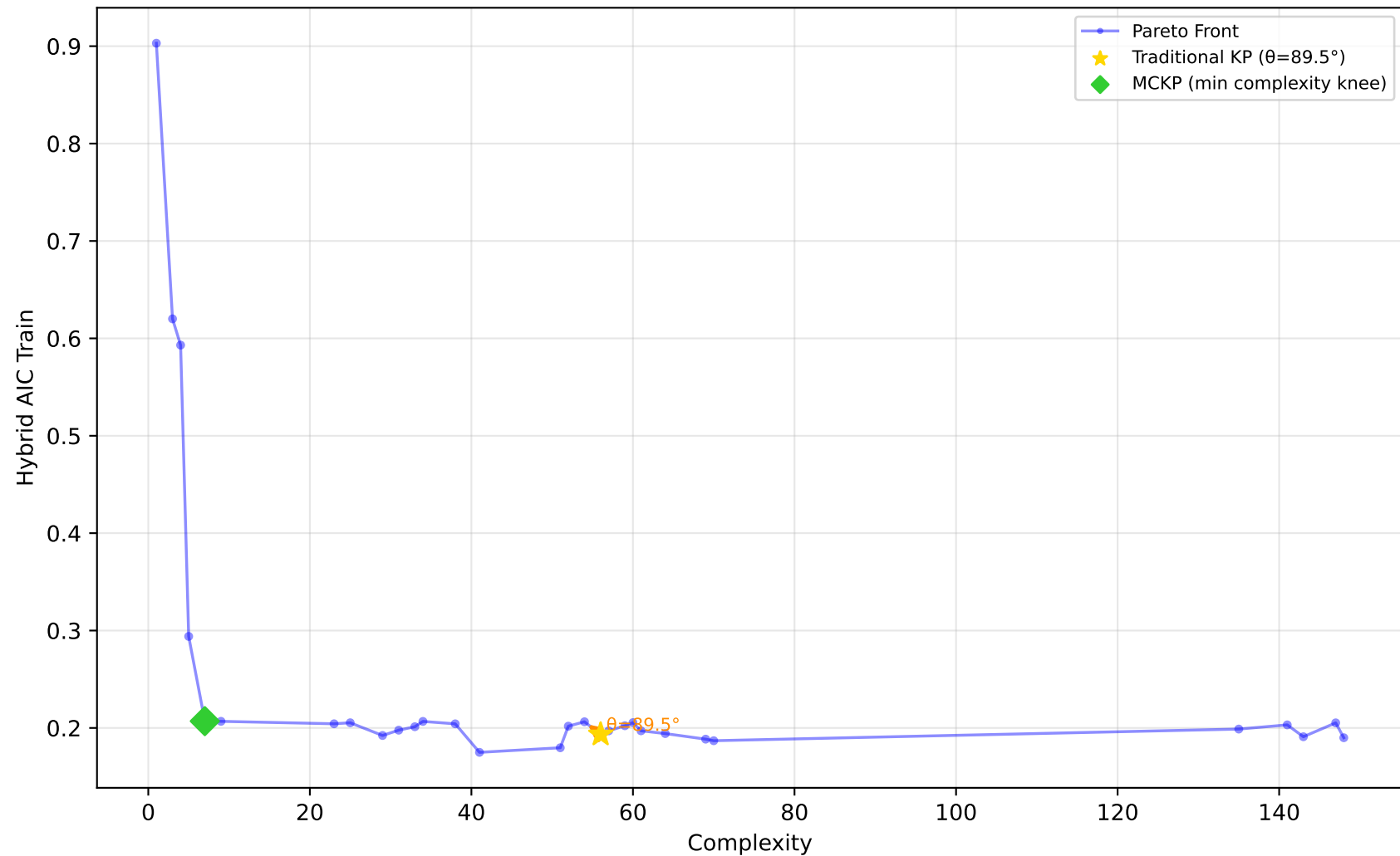
519_vinnie - Run 3 - MVP - Hybrid AIC Train \lambda_1=1.00, \lambda_2=0.00, \lambda_3=1.00 | Difficulty: 1.00 | Method: hmr
