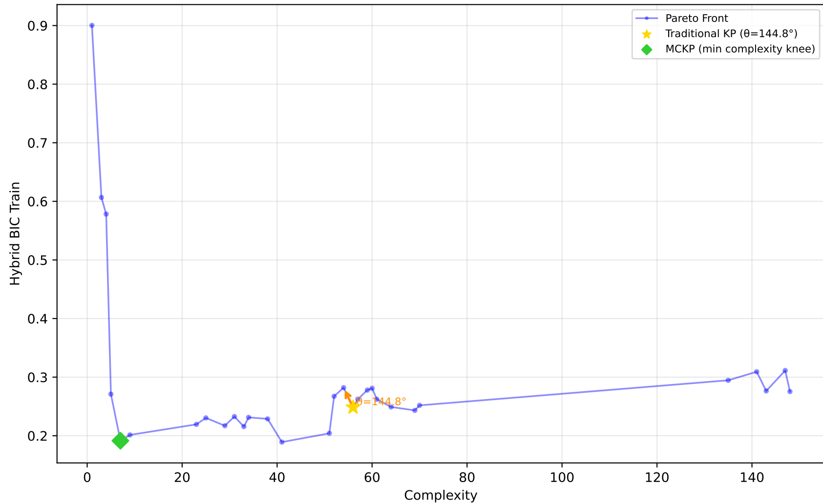
519_vinnie - Run 3 - MVP - Hybrid BIC Train \lambda_1=1.00, \lambda_2=0.00, \lambda_3=1.00 | Difficulty: 1.00 | Method: hmr
