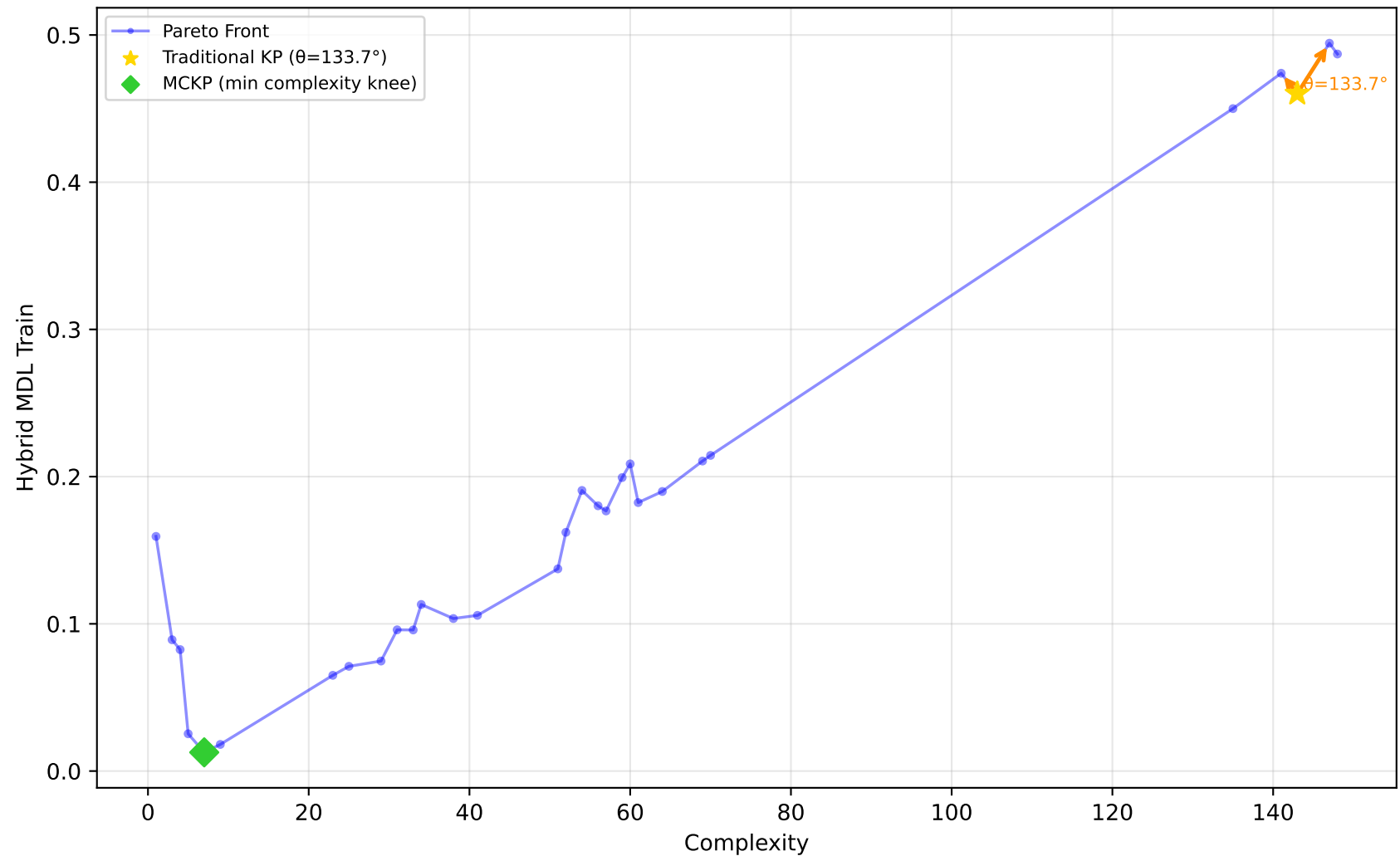
519_vinnie - Run 3 - MVP - Hybrid MDL Train \lambda_1=0.00, \lambda_2=0.10, \lambda_3=0.00 | Difficulty: 1.00 | Method: hmr
