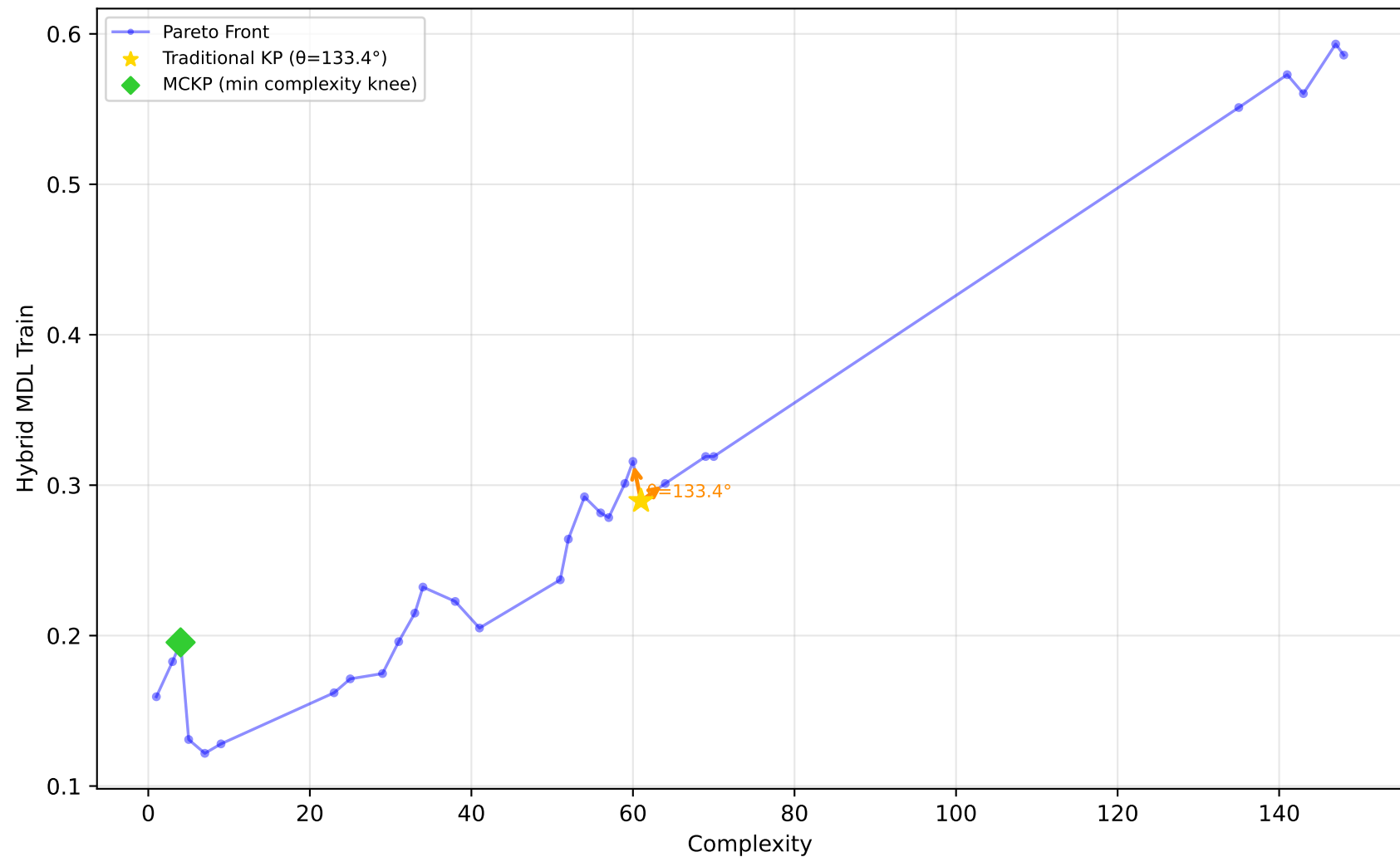
519_vinnie - Run 3 - MVP - Hybrid MDL Train \lambda_1=1.00, \lambda_2=0.00, \lambda_3=1.00 | Difficulty: 1.00 | Method: hmr
