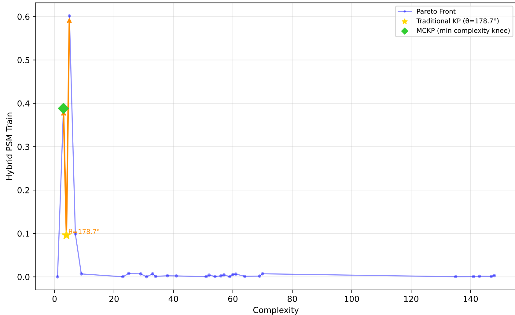
519_vinnie - Run 3 - MVP - Hybrid PSM Train \lambda_1=0.00, \lambda_2=0.10, \lambda_3=0.00 | Difficulty: 1.00 | Method: hmr
