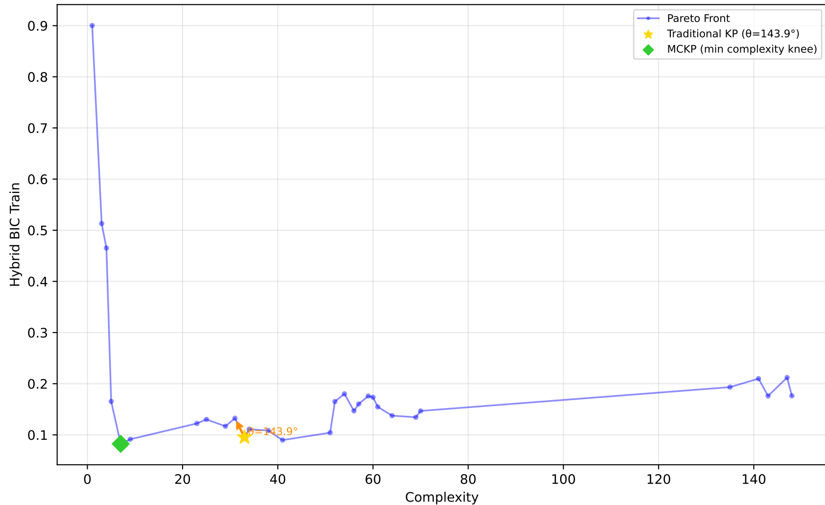
519_vinnie - Run 3 - SVP - Hybrid BIC Train \lambda_1=0.00, \lambda_2=0.00, \lambda_3=0.00 | Difficulty: 1.00 | Method: hmr
