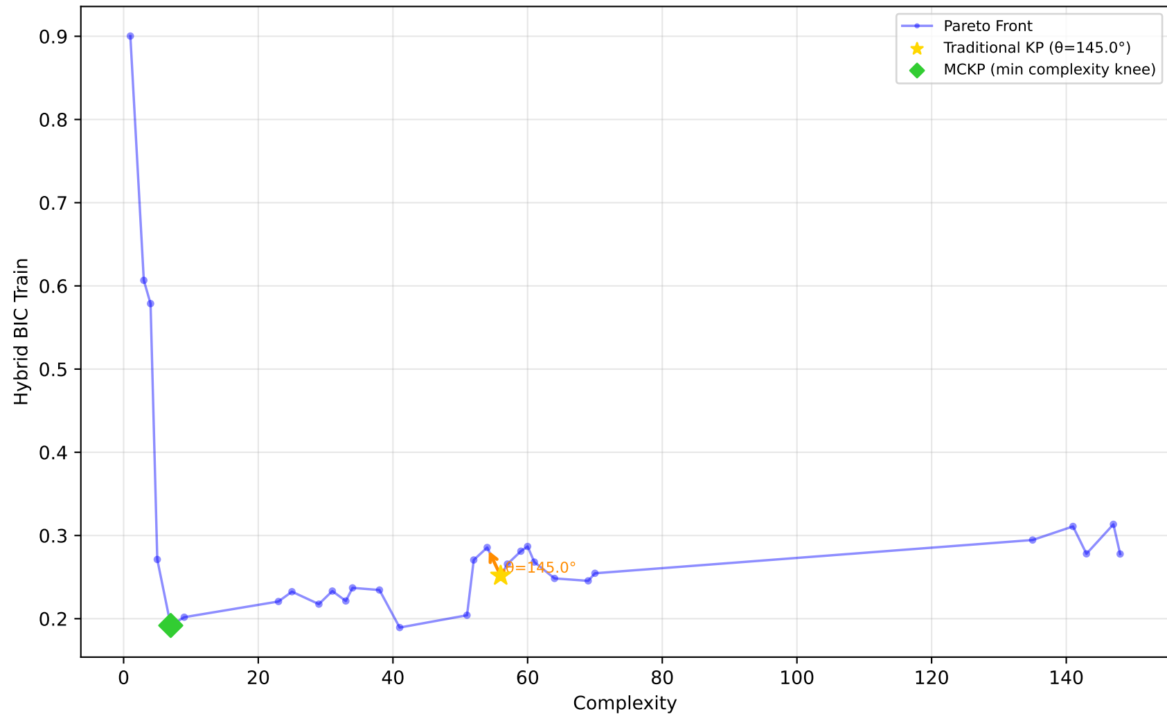
519_vinnie - Run 3 - SVP - Hybrid BIC Train \lambda_1=1.00, \lambda_2=1.00, \lambda_3=1.00 | Difficulty: 1.00 | Method: hmr
