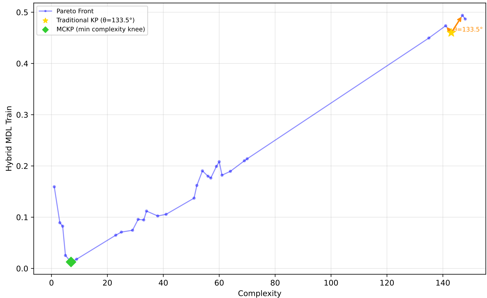
519_vinnie - Run 3 - SVP - Hybrid MDL Train \lambda_1=0.00, \lambda_2=0.00, \lambda_3=0.00 | Difficulty: 1.00 | Method: hmr
