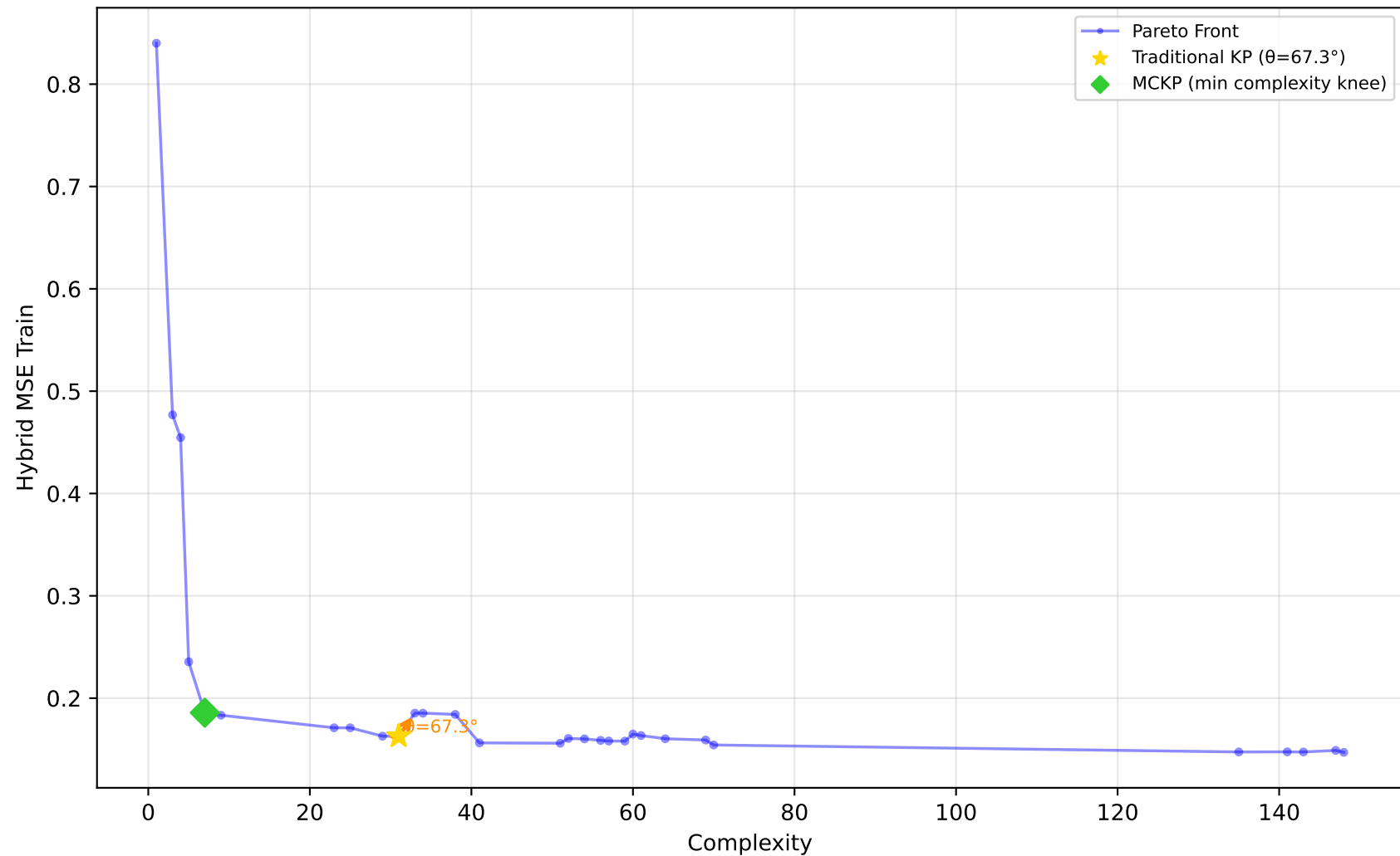
519_vinnie - Run 3 - SVP - Hybrid MSE Train \lambda_1=1.00, \lambda_2=1.00, \lambda_3=1.00 | Difficulty: 1.00 | Method: hmr
